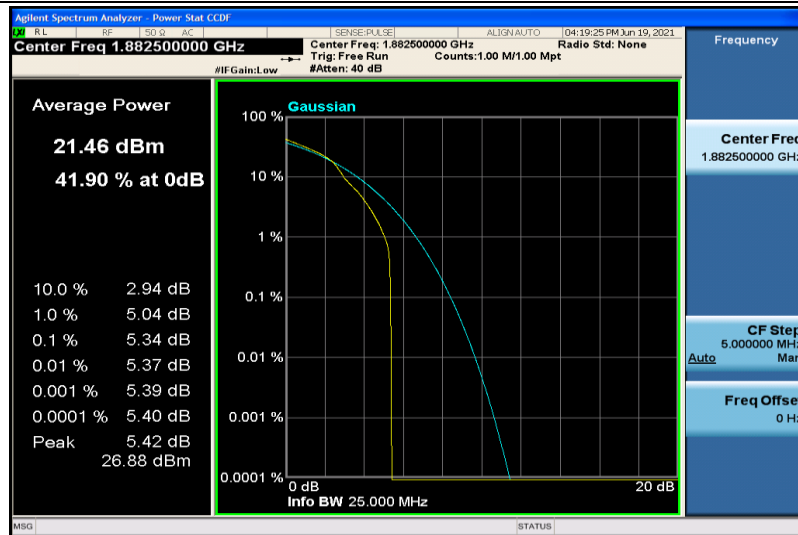
Band25-5MHz-16QAM-26365-1RB#0
