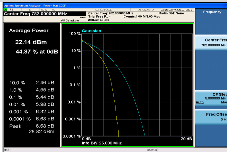
Band13-10MHz-QPSK-23230-50RB#0
