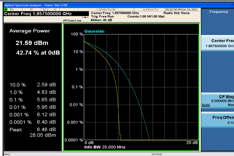
Band25-15MHz-QPSK-26115-75RB#0
