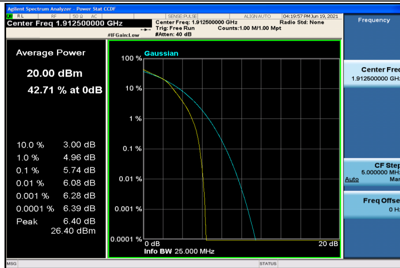
Band25-5MHz-16QAM-26665-25RB#0
