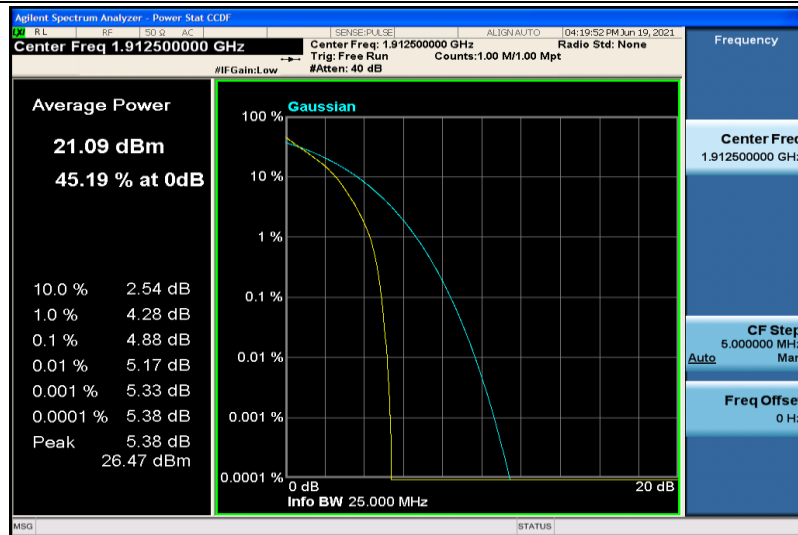
Band25-5MHz-QPSK-26665-25RB#0
