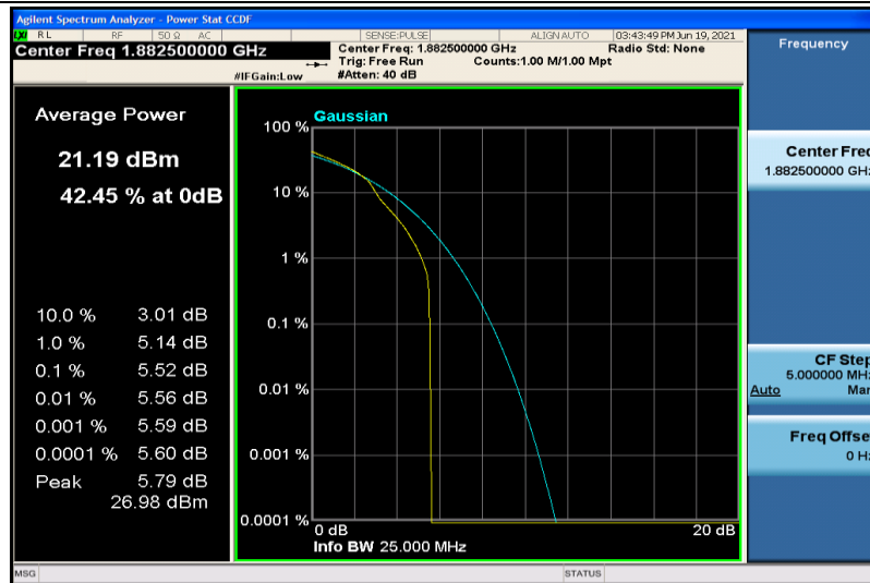
Band25-1.4MHz-16QAM-26365-1RB#0
