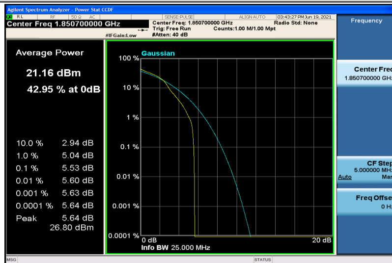
Band25-1.4MHz-16QAM-26047-1RB#0
