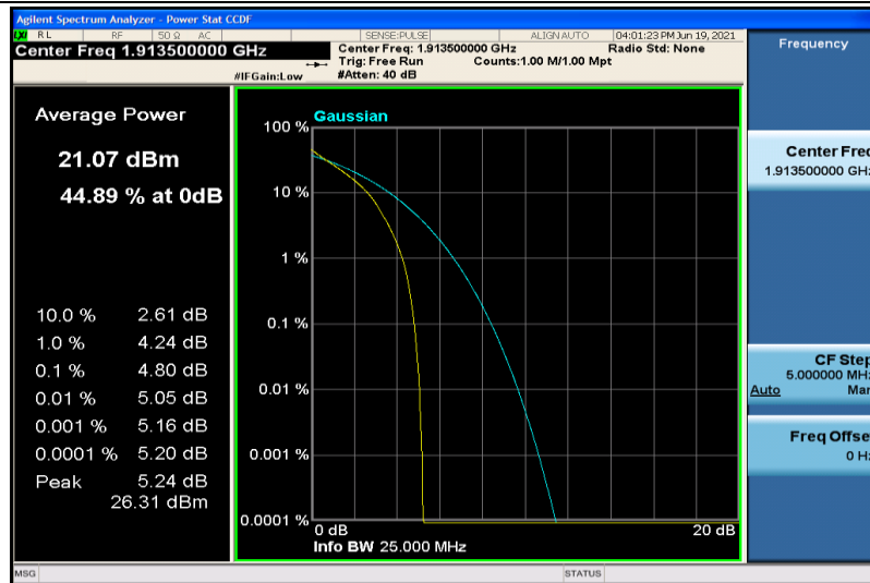
Band25-3MHz-QPSK-26675-15RB#0
