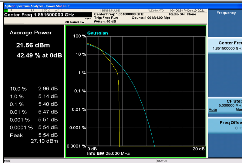
Band25-3MHz-16QAM-26055-1RB#0
