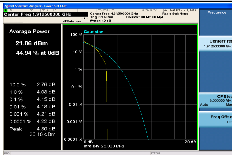
Band25-5MHz-QPSK-26665-1RB#0
