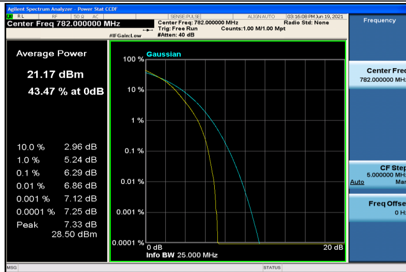
Band13-10MHz-16QAM-23230-50RB#0
