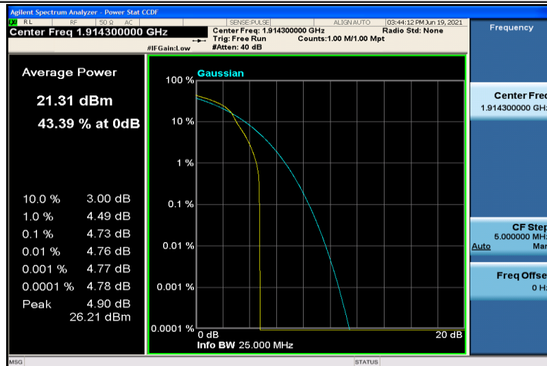
Band25-1.4MHz-16QAM-26683-1RB#0
