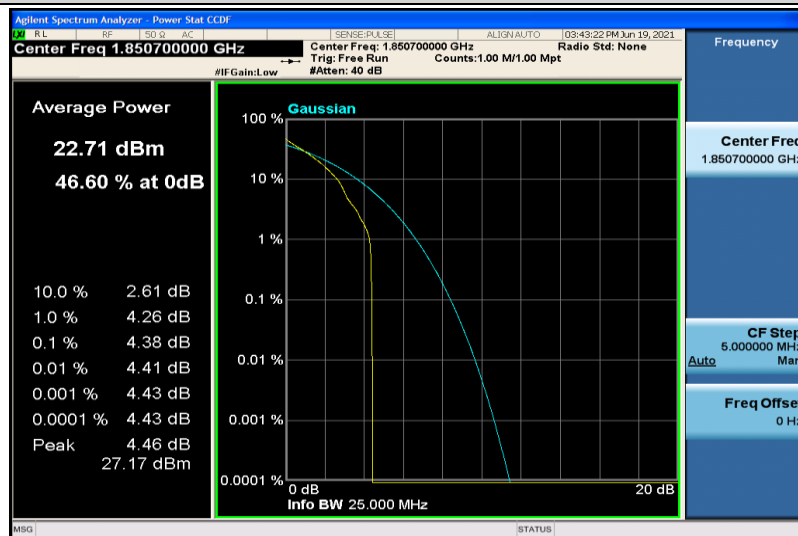
Band25-1.4MHz-QPSK-26047-1RB#0
