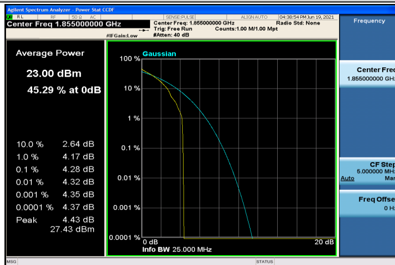
Band25-10MHz-QPSK-26090-1RB#0
