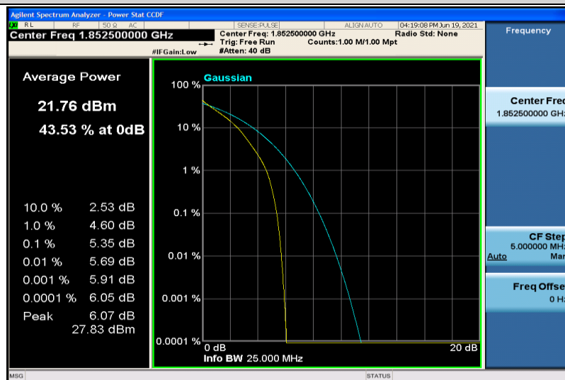
Band25-5MHz-QPSK-26065-25RB#0
