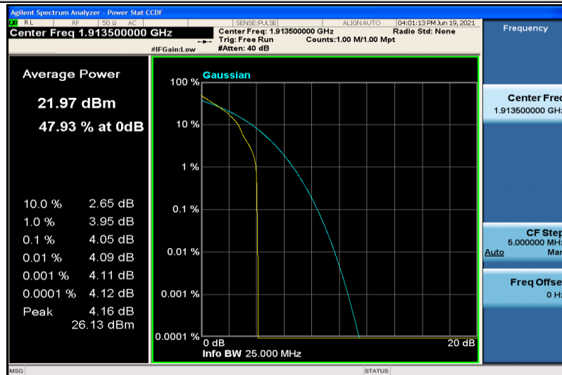
Band25-3MHz-QPSK-26675-1RB#0
