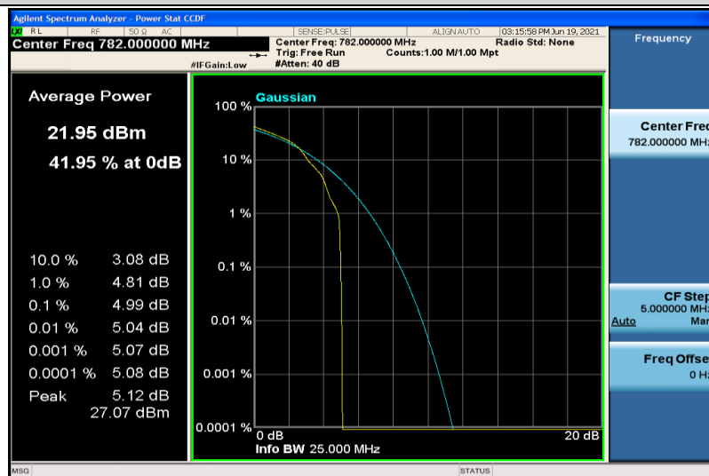
Band13-10MHz-16QAM-23230-1RB#0
