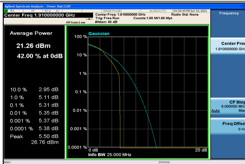
Band25-10MHz-16QAM-26640-1RB#0
