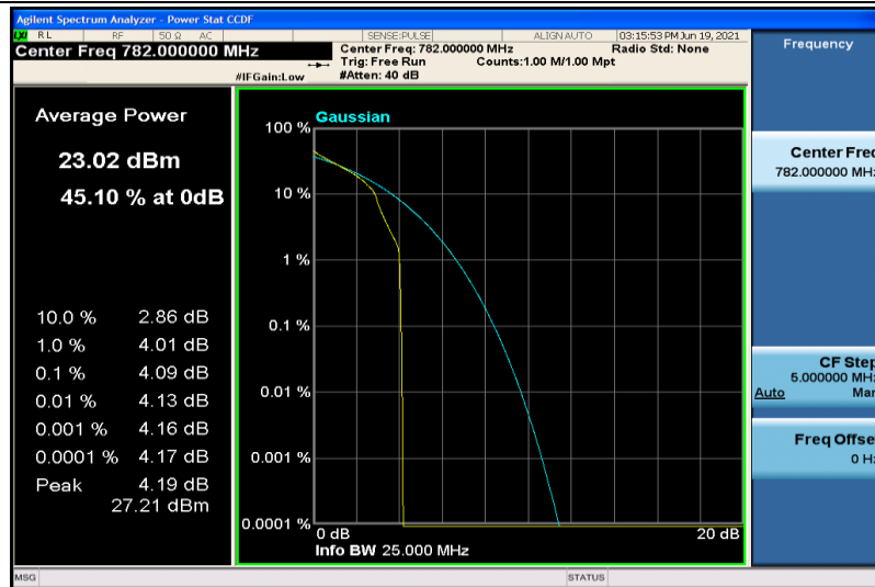
Band13-10MHz-QPSK-23230-1RB#0
