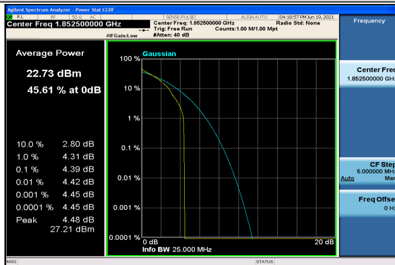
Band25-5MHz-QPSK-26065-1RB#0
