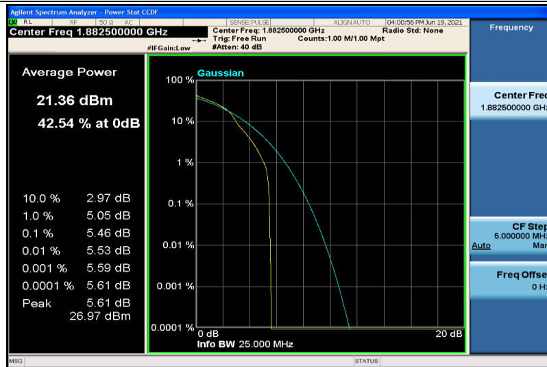
Band25-3MHz-16QAM-26365-1RB#0
