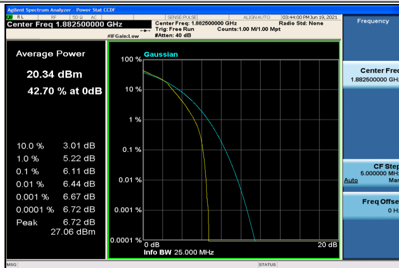
Band25-1.4MHz-16QAM-26365-6RB#0
