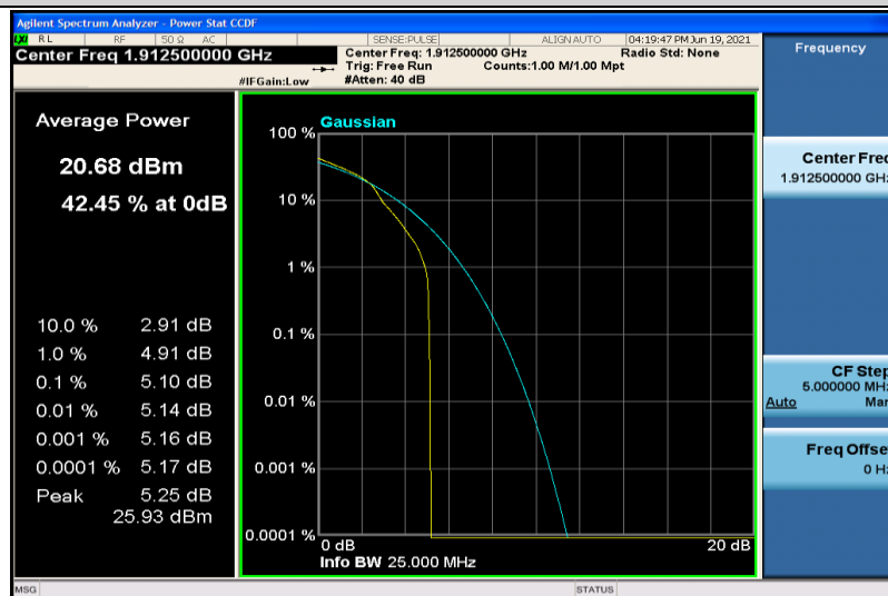
Band25-5MHz-16QAM-26665-1RB#0
