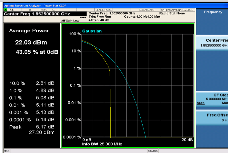
Band25-5MHz-16QAM-26065-1RB#0
