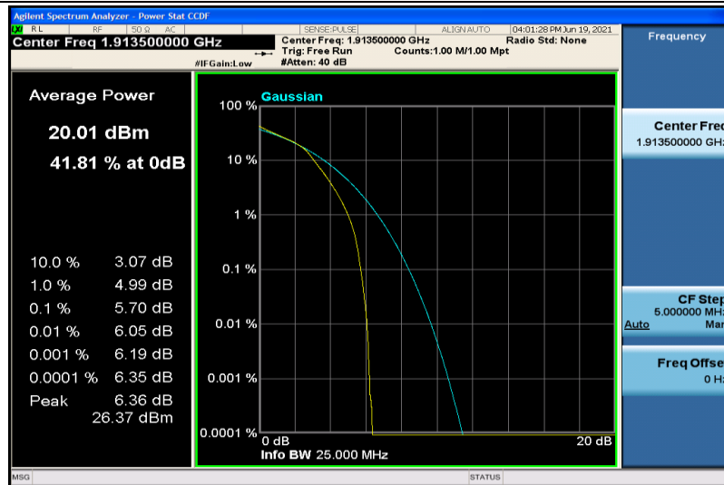
Band25-3MHz-16QAM-26675-15RB#0
