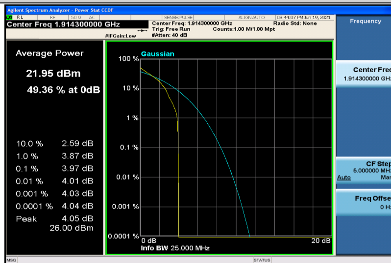
Band25-1.4MHz-QPSK-26683-1RB#0
