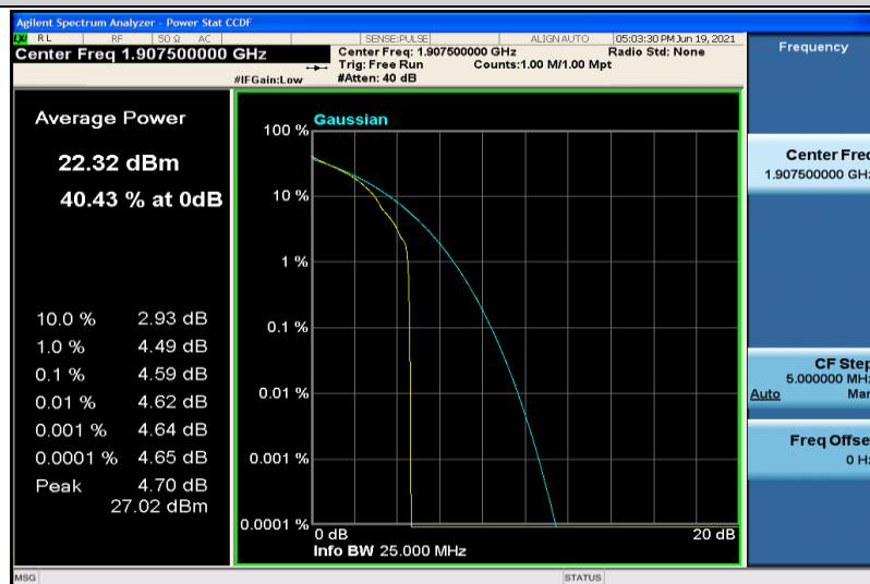
Band25-15MHz-QPSK-26615-1RB#0
