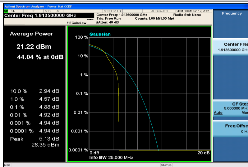
Band25-3MHz-16QAM-26675-1RB#0
