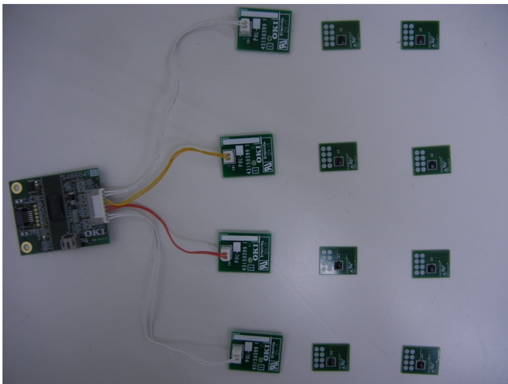
RFID Reader/Writer Board and RF Antenna Board of Reader/Writer module (4666411A)
