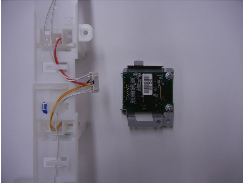
RFID Reader/Write Board is screwed to shield sheat metal
