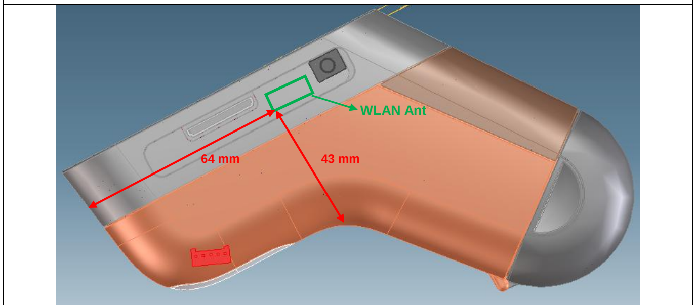
EUT – Right Side View
