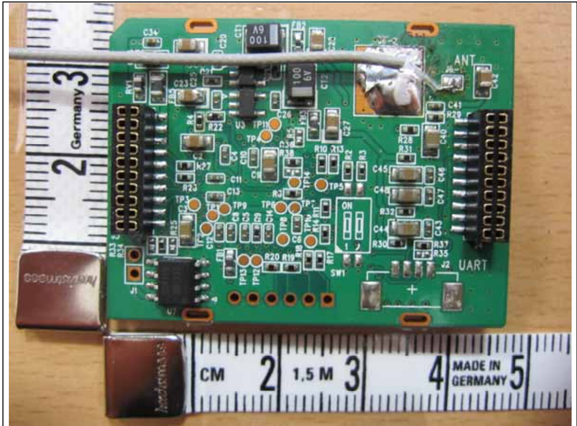
RF Board - Rear
