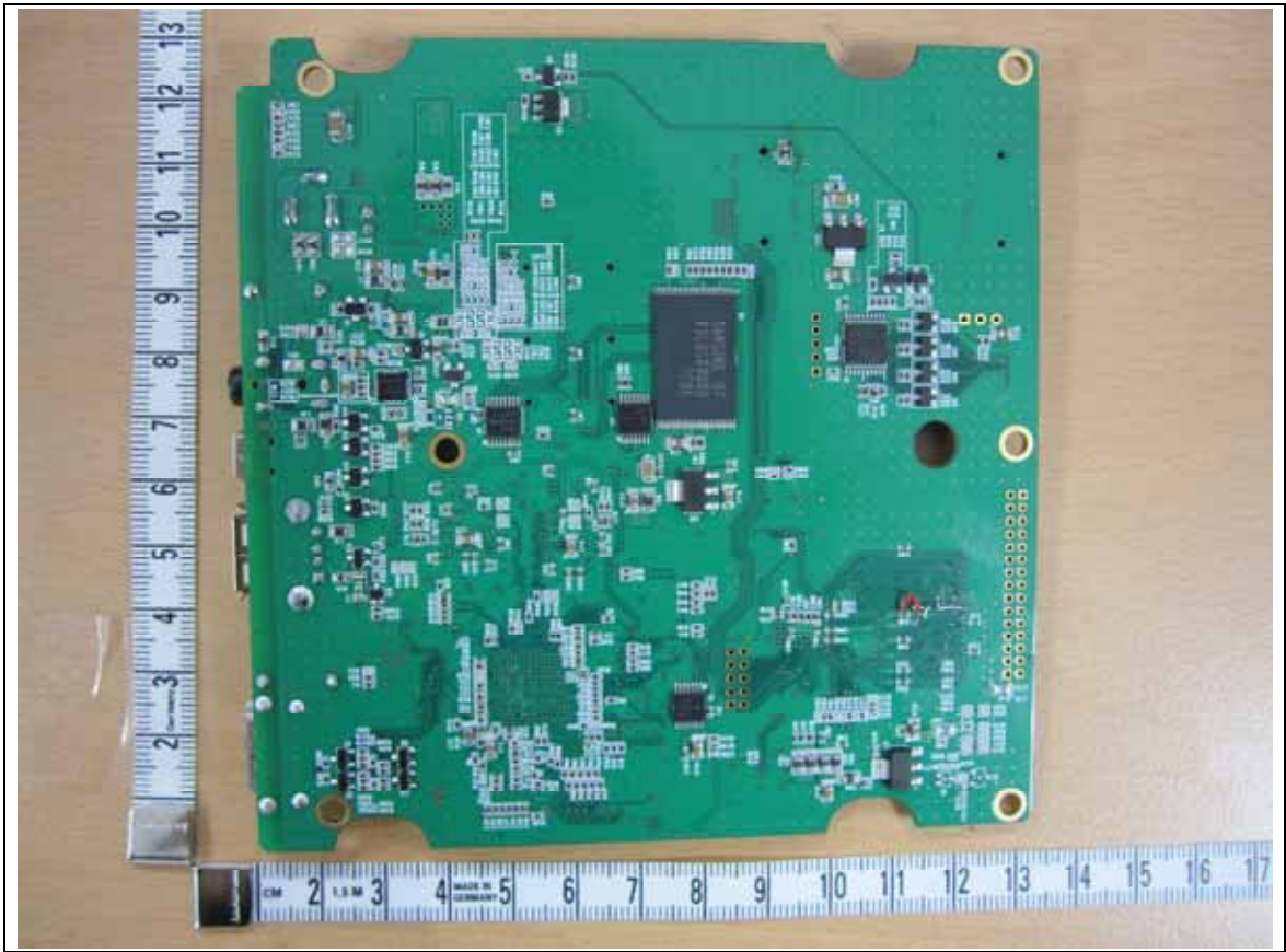
MainBoard - Rear
