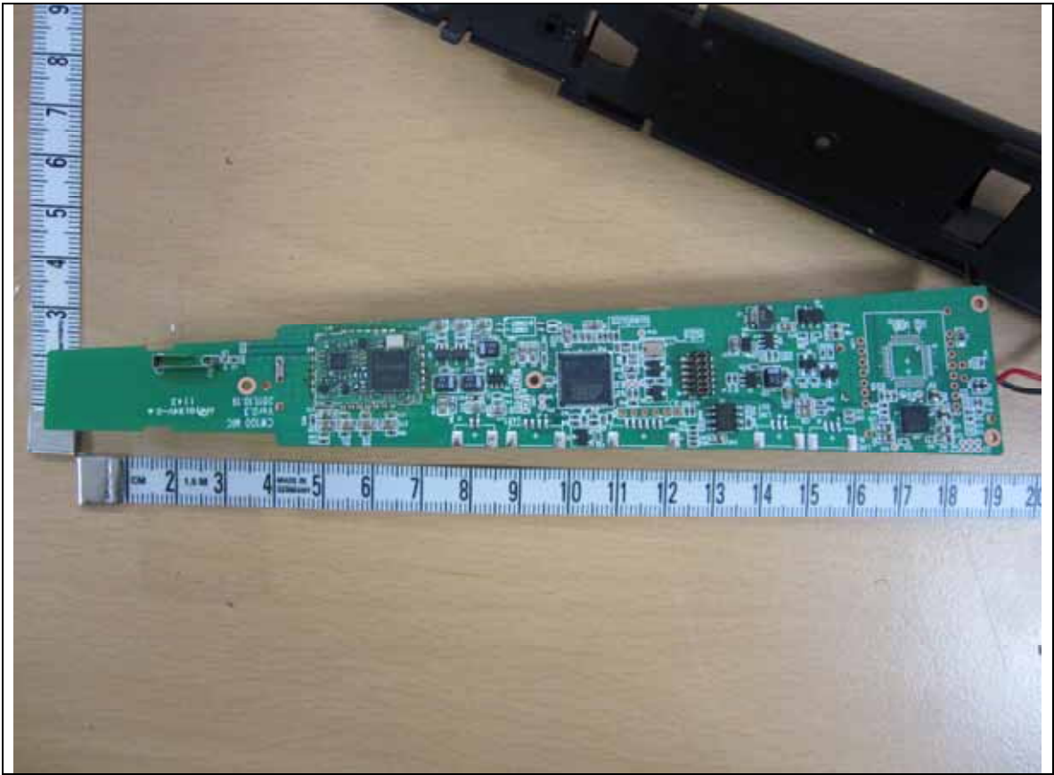
MainBoard - Rear
