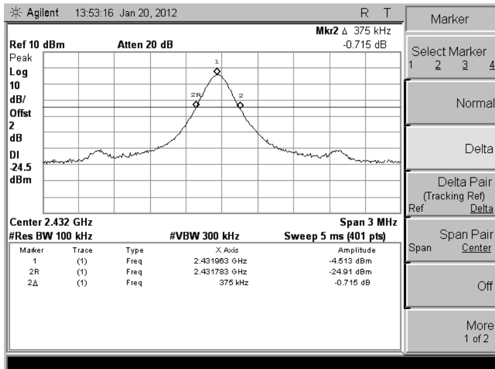
CH MID
