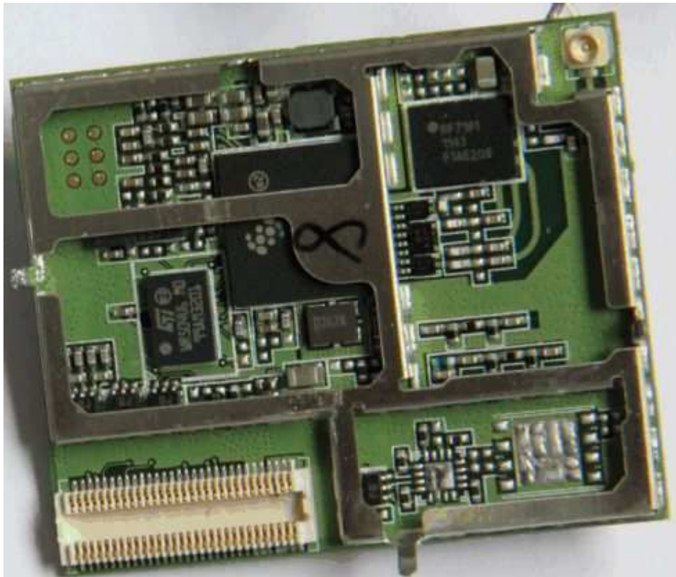
Fig. 6: Internal view
