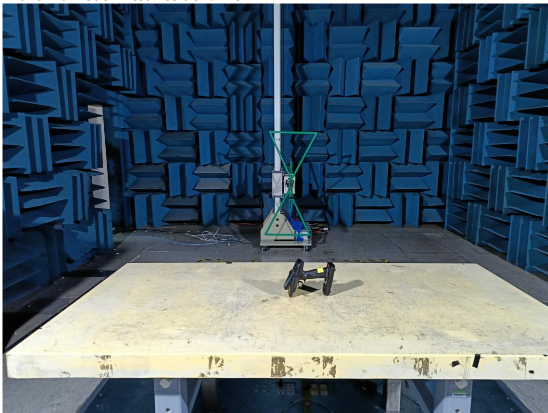
Transmit Mode - Test Position: Lie
