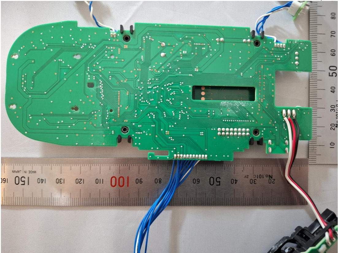
Figure 36 PCB, Back View
