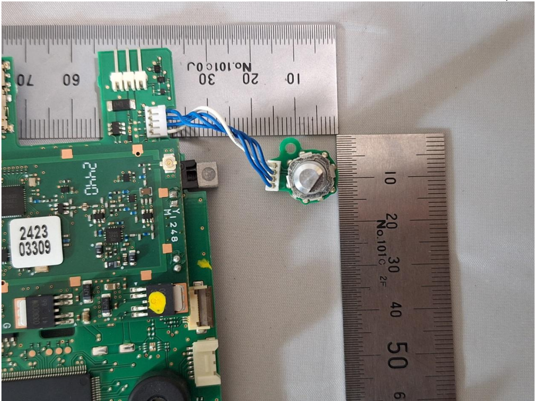
Figure 33 PCB, Front View
