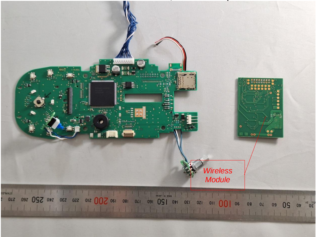
Figure 37 PCB, Front View (Removed Wireless Module)
