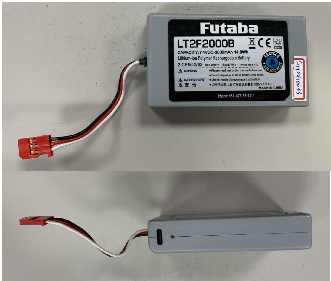
Figure 12 LiPo Battery View
