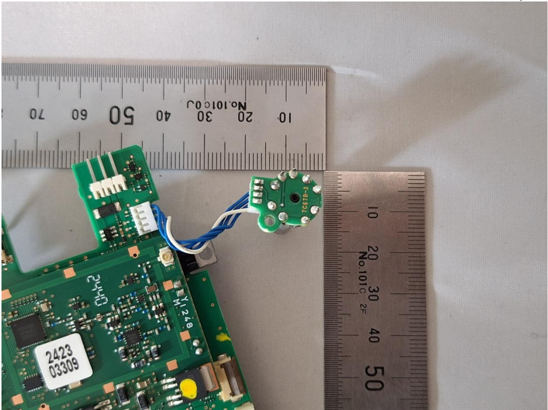
Figure 34 PCB, Back View
