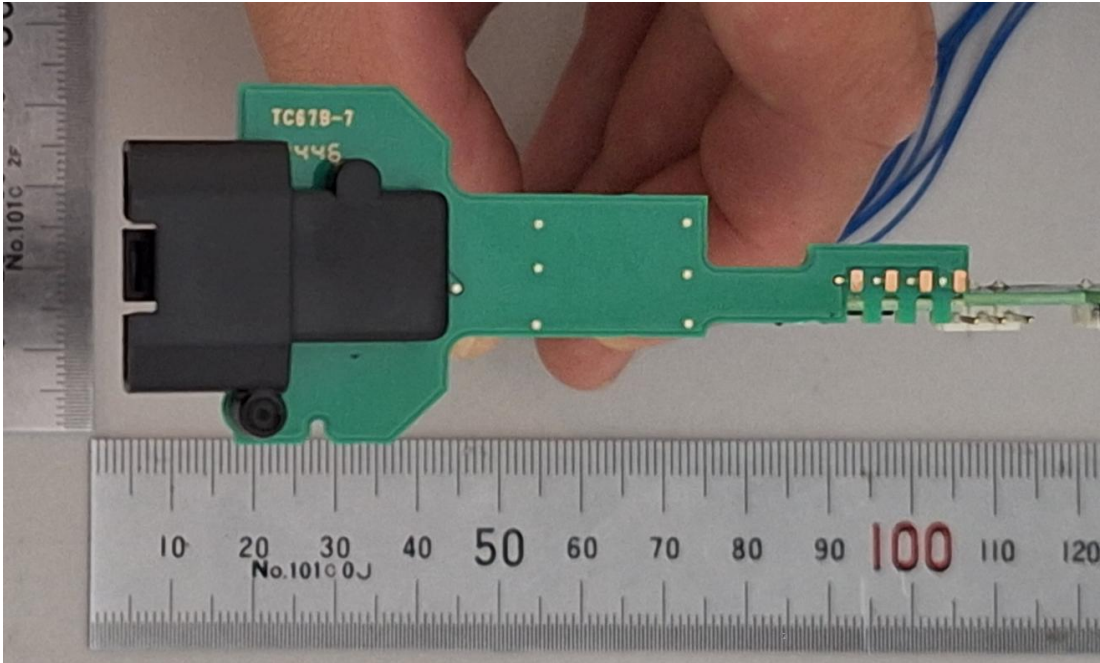
Figure 28 PCB, Back View
