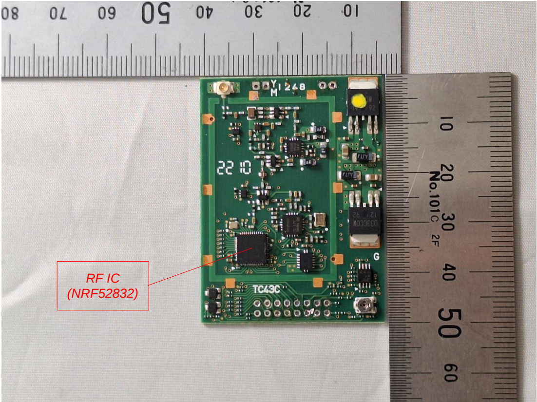
Figure 39 Wireless Module, Front View
