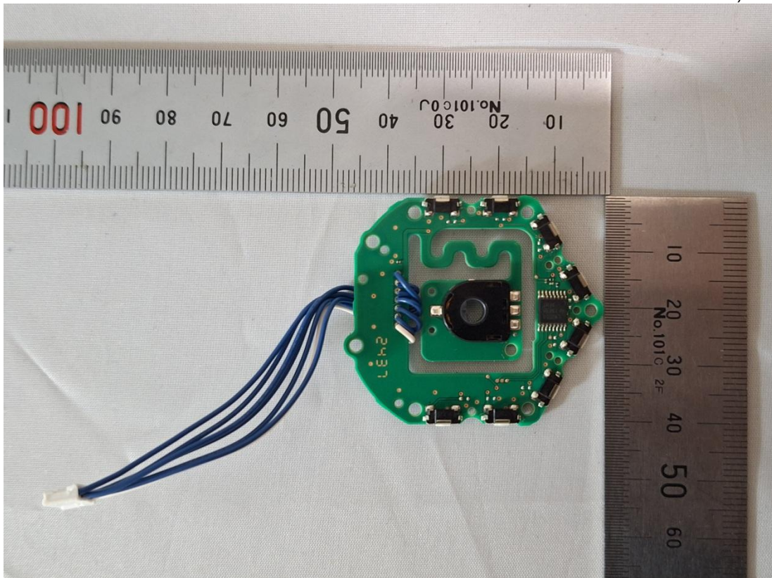
Figure 30 PCB, Back View
