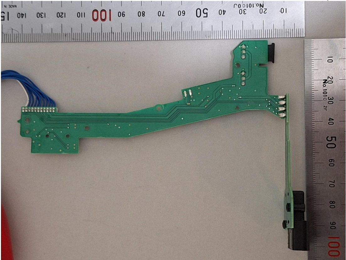
Figure 25 PCB, Front View
