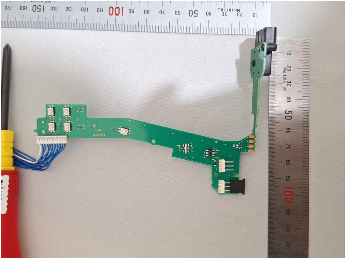
Figure 26 PCB, Back View
