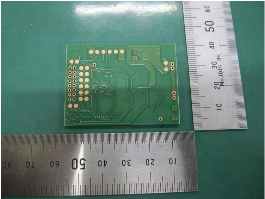
Figure 38 Wireless Module, Back View
