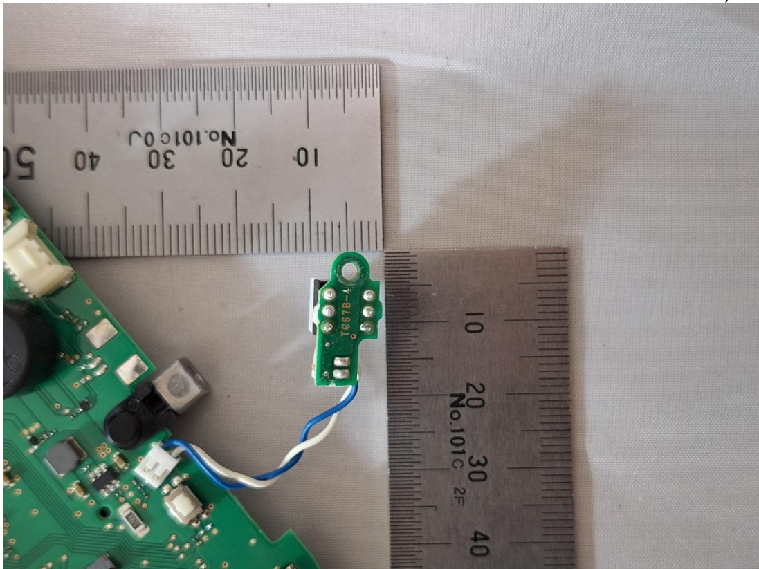
Figure 32 PCB, Back View
