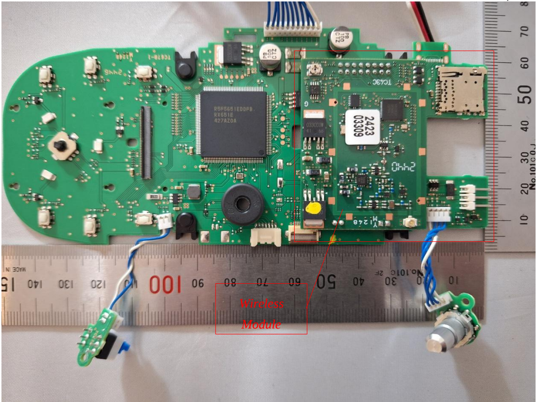
Figure 35 PCB, Front View
