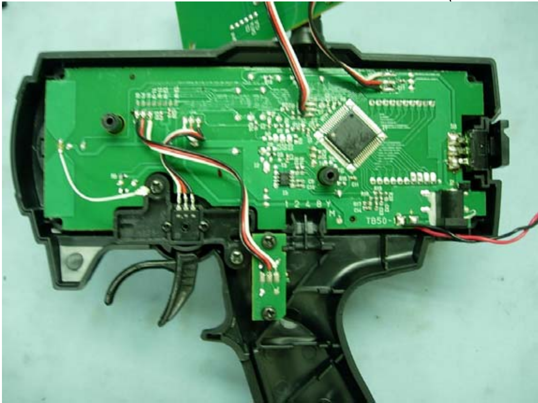
Figure 14 Internal View (Control Boards)
