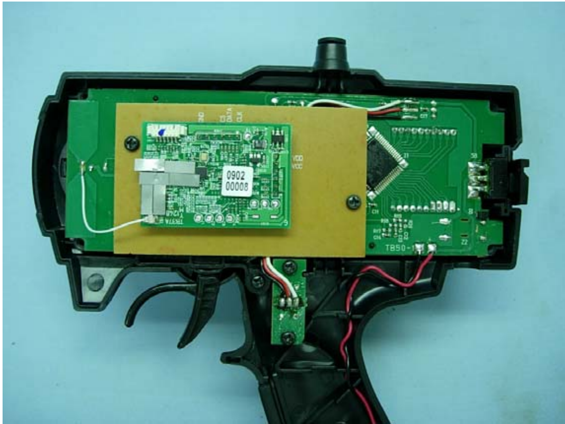
Figure 8 Internal View
