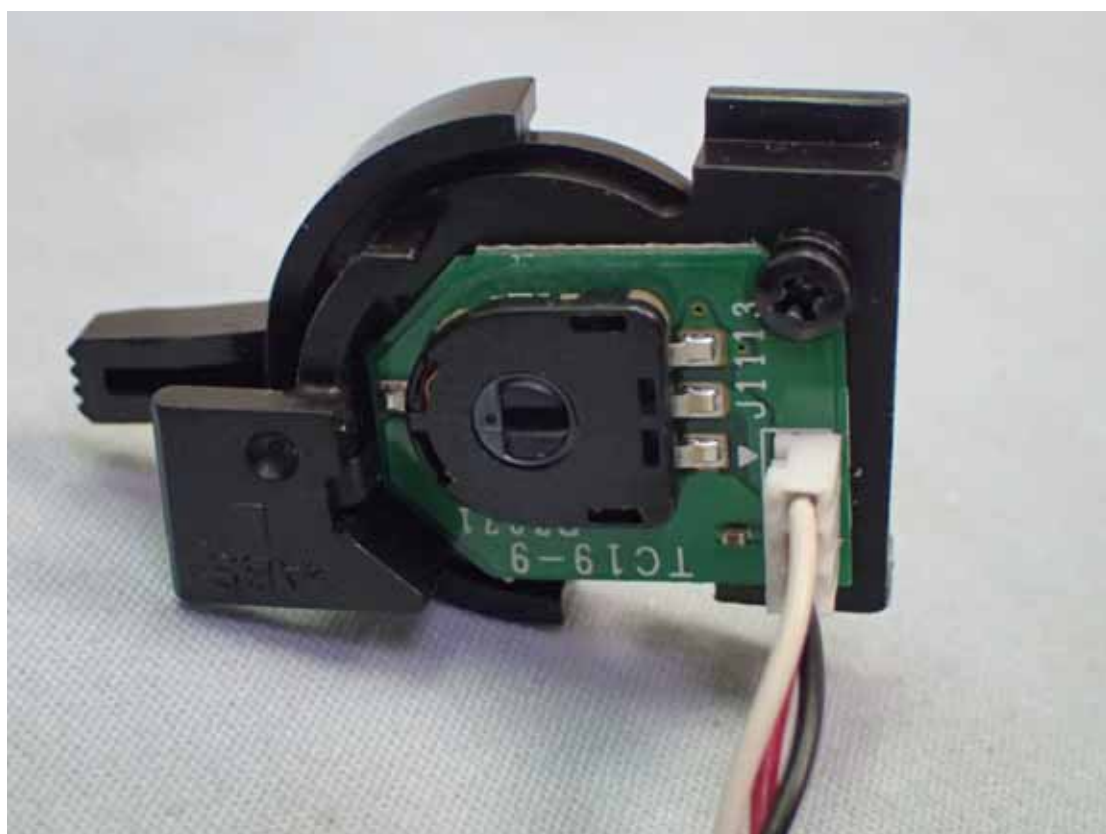
Figure 18 Internal View
