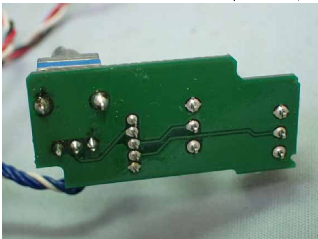
Figure 22 Internal View (Control Board, Front View)
