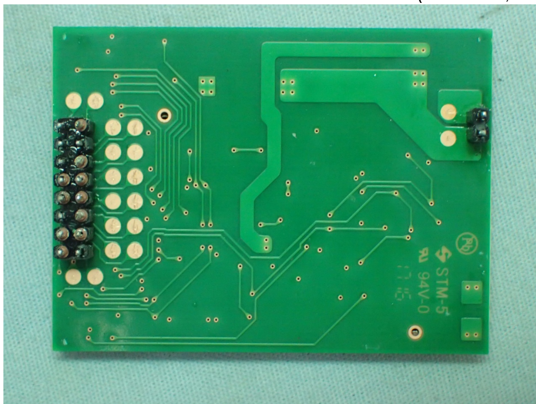
Figure 29 Internal View (RF Module, Back View)
