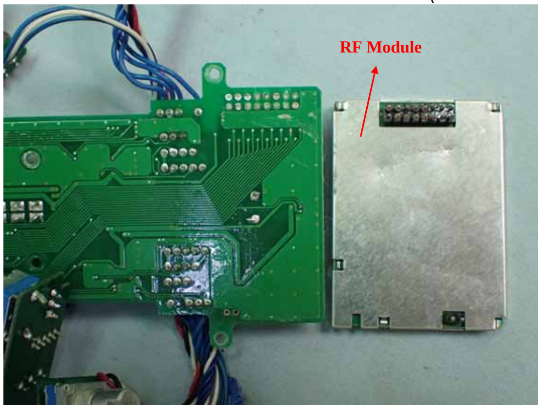
Figure 27 Internal View (Removed RF Module)
