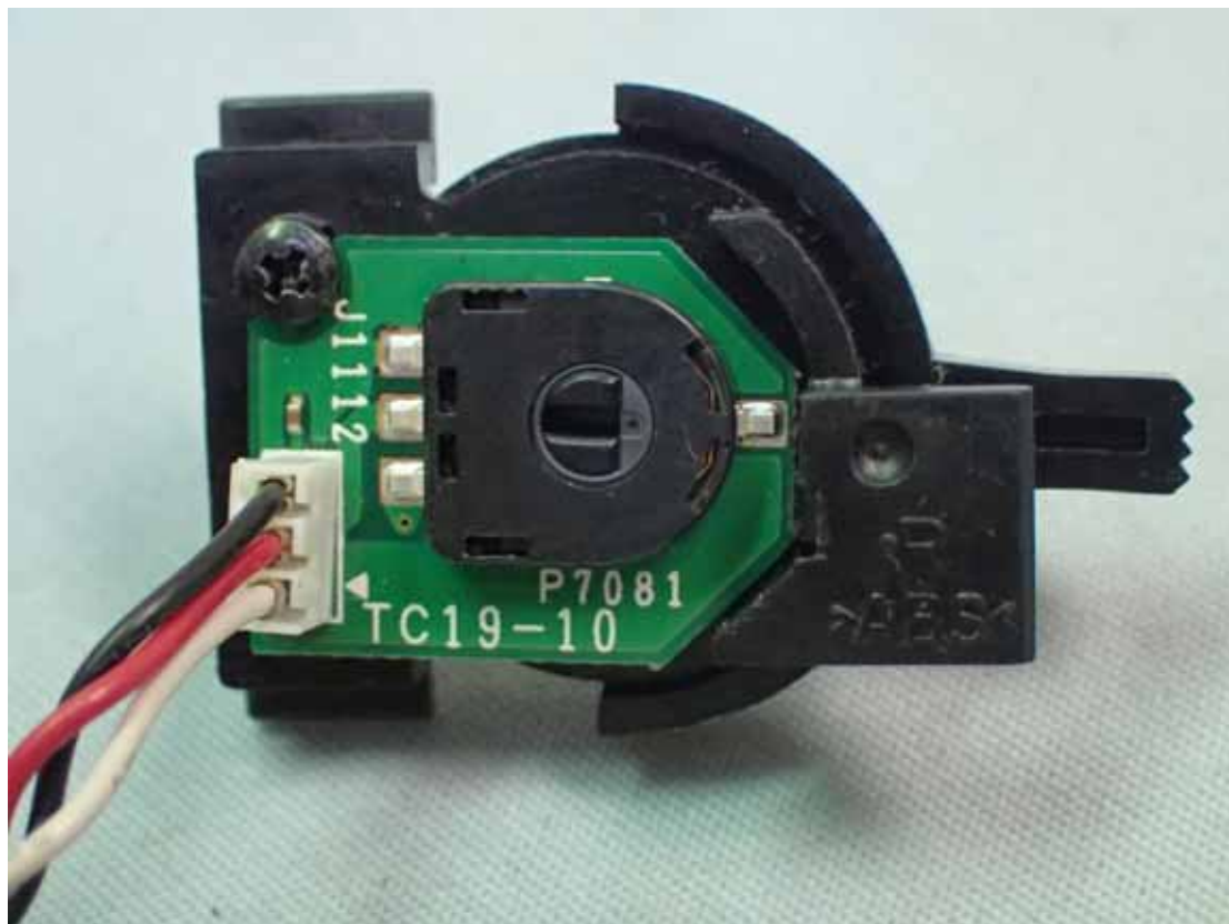
Figure 13 Internal View
