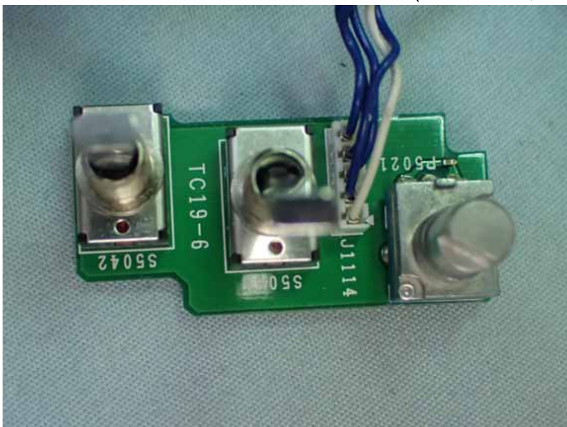
Figure 16 Internal View (Control Board, Front View)
