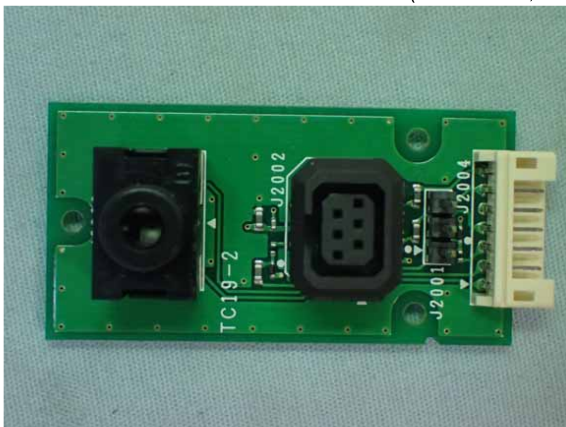
Figure 10 Internal View (I/O Port Board, Front View)
