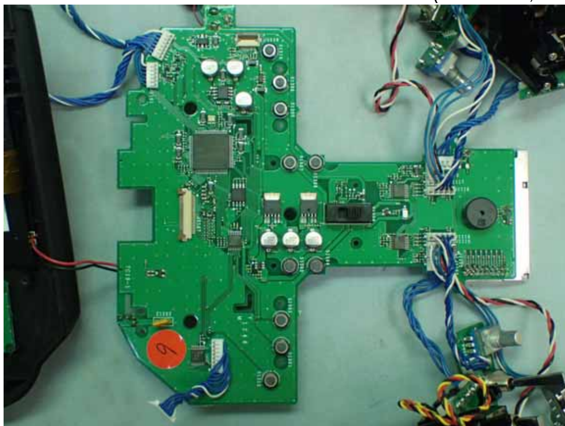
Figure 25 Internal View (Main Board, Front View)
