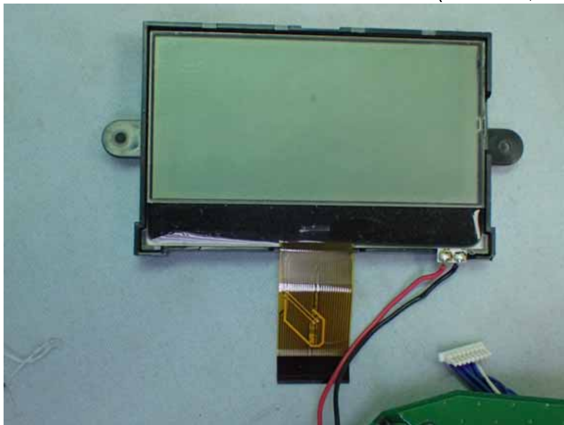
Figure 35 Internal View (LCD Panel, Front View)
