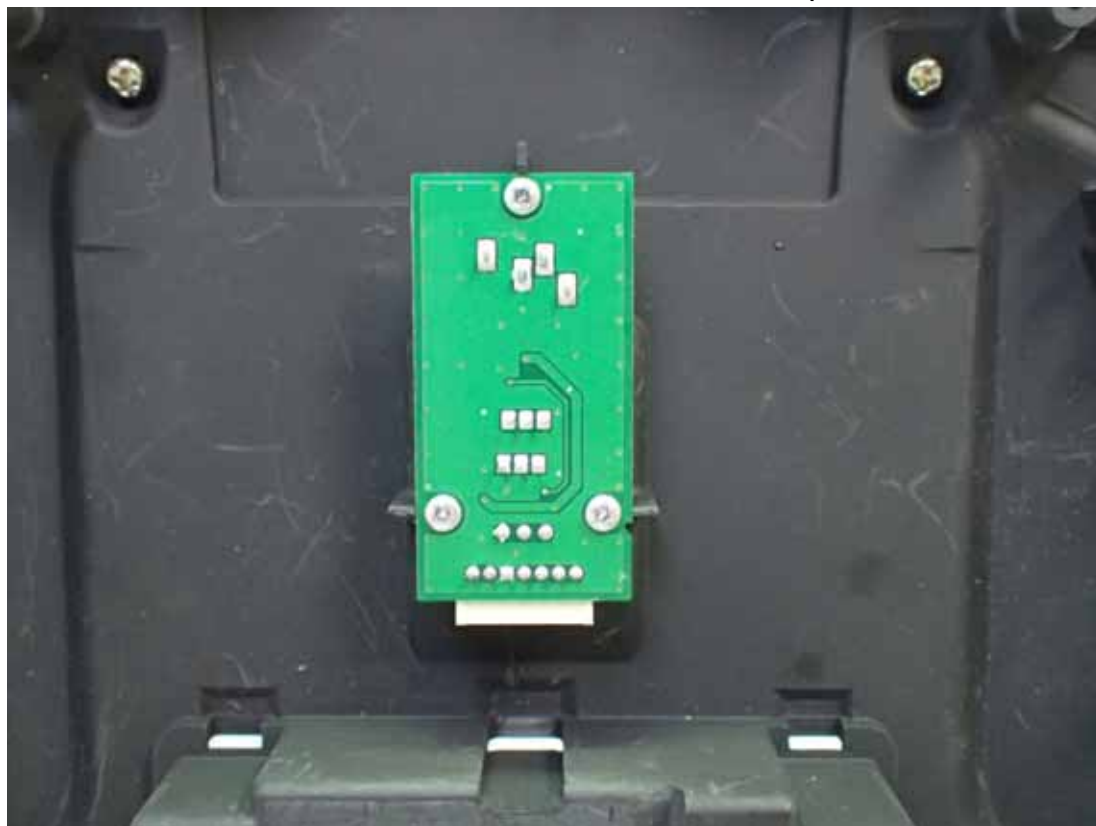
Figure 9 Internal View (I/O Port Board, Back View)
