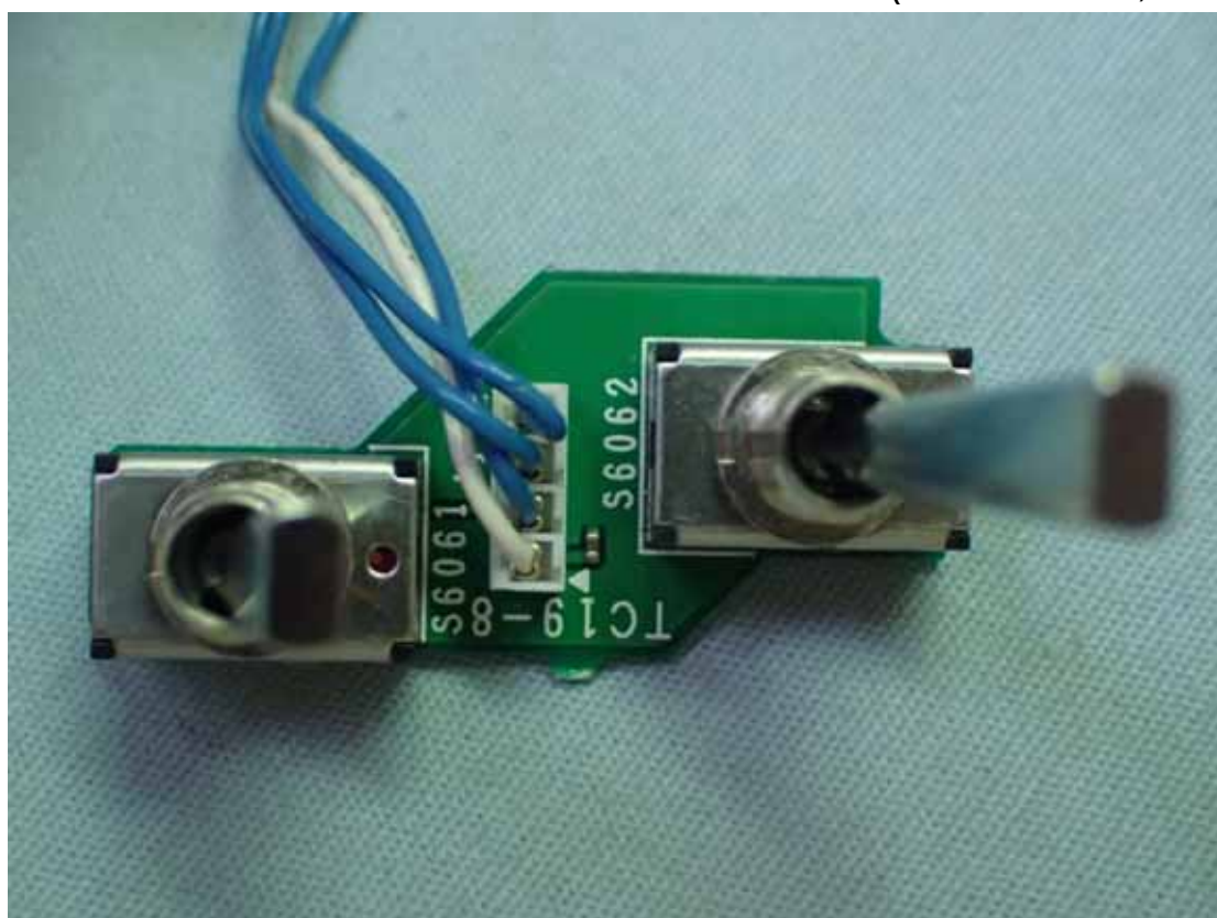
Figure 14 Internal View (Control Board, Front View)
