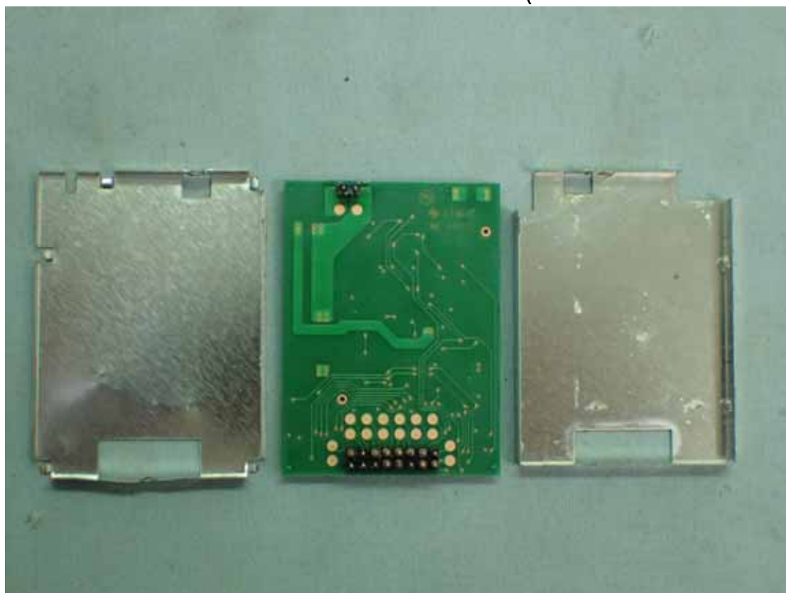
Figure 28 Internal View (Removed RF Module's Covers)
