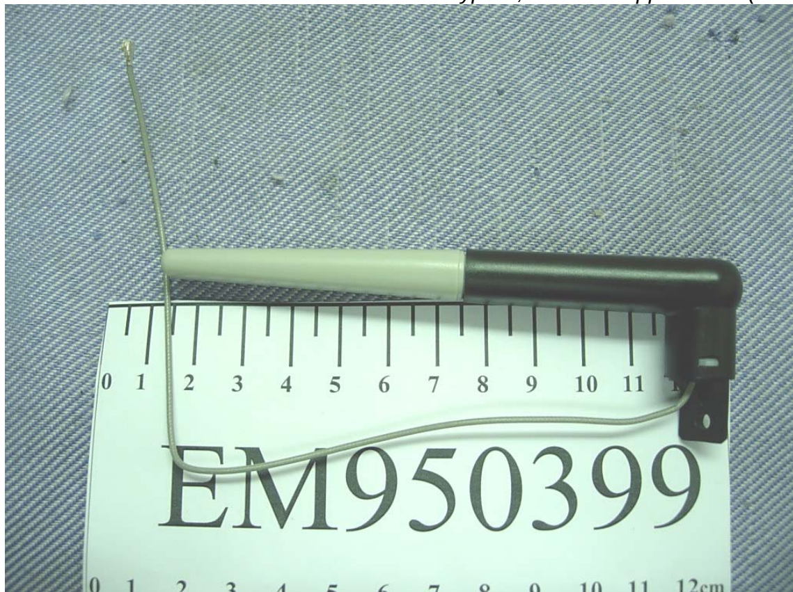
Figure 4 Antenna Type B, General Appearance (Side View)
