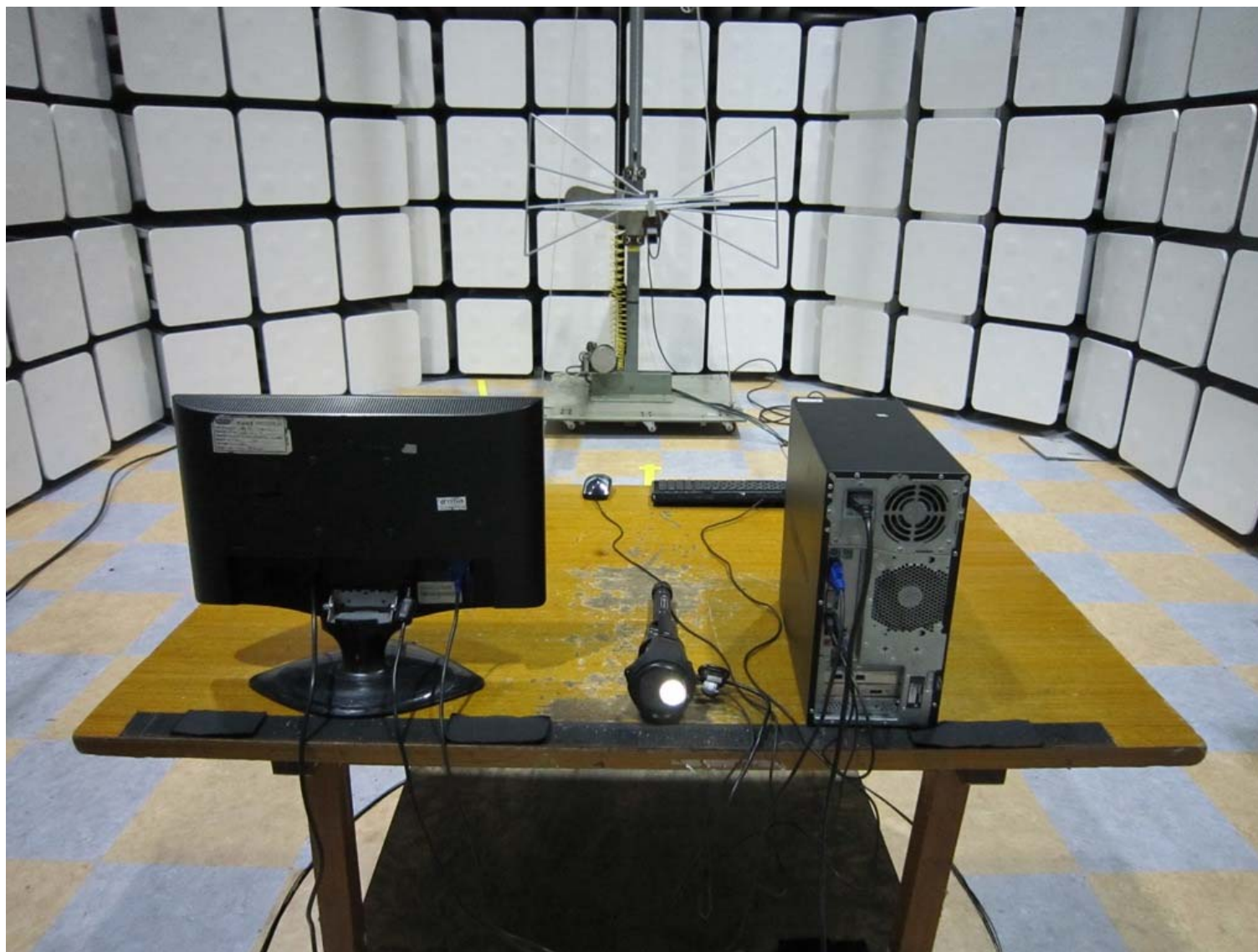
Radiated_30 MHz to 1 GHz_USB Data Up/Down & LED Lighting Mode_Rear View
