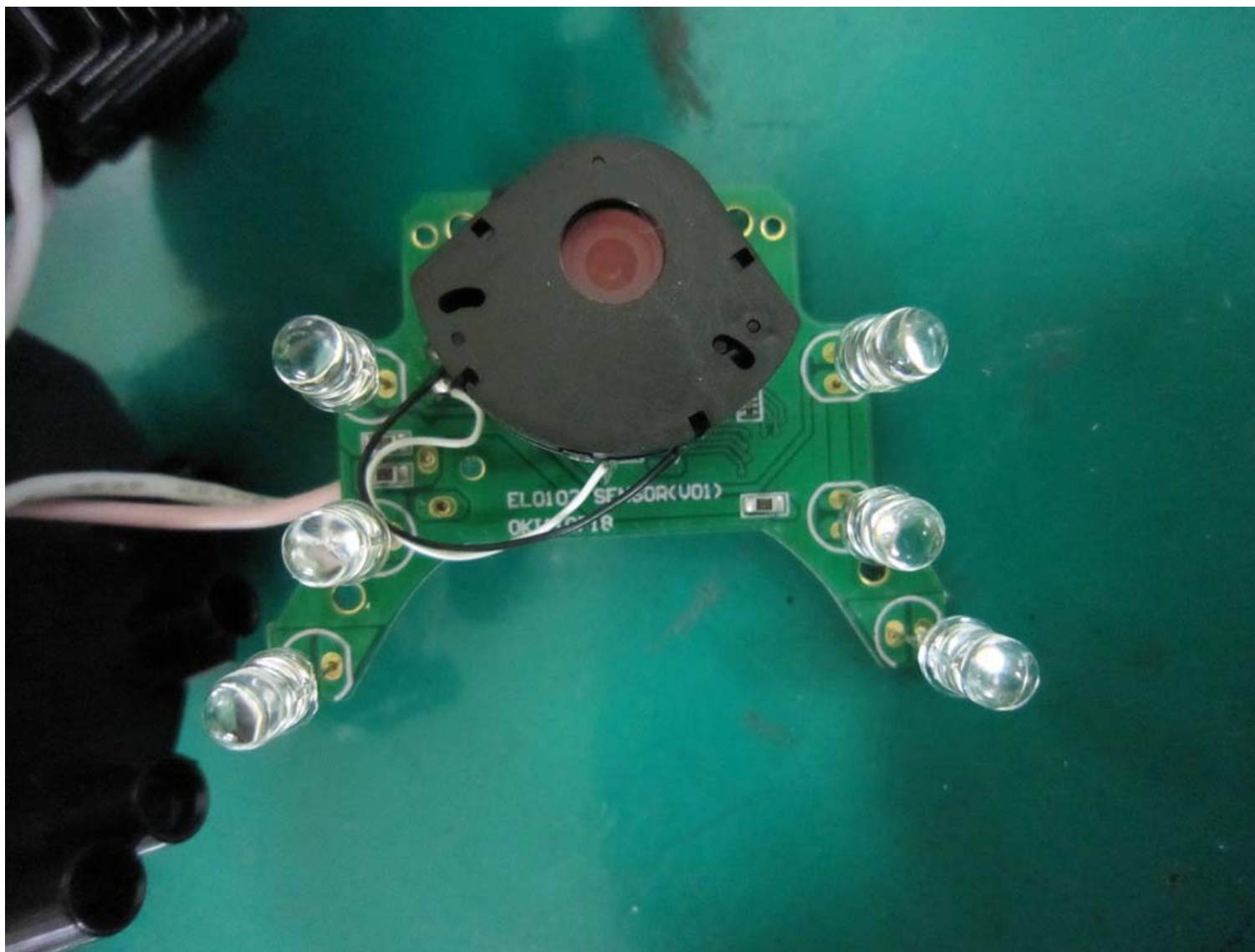
GCF-200_Camera Board(Front View)
