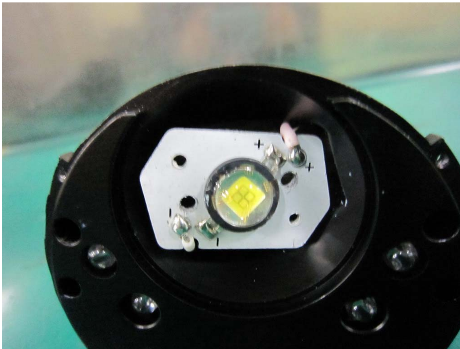
GCF-200_LED Board(Front View)
