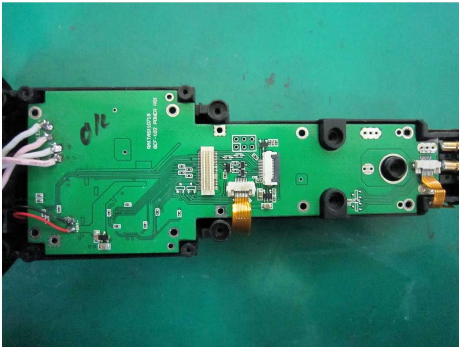
GCF-200_Power Board(Rear View)
