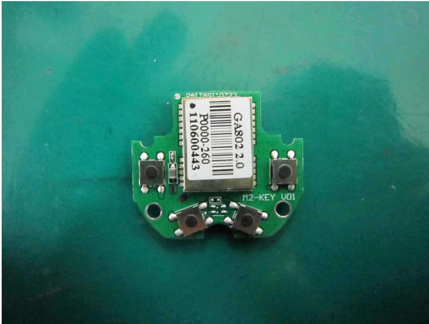
GCF-200_Button Board(Front View)
