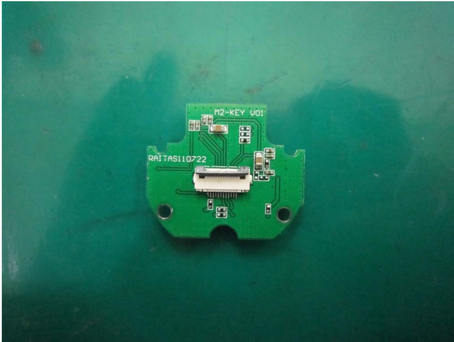
GCF-200_Button Board(Rear View)
