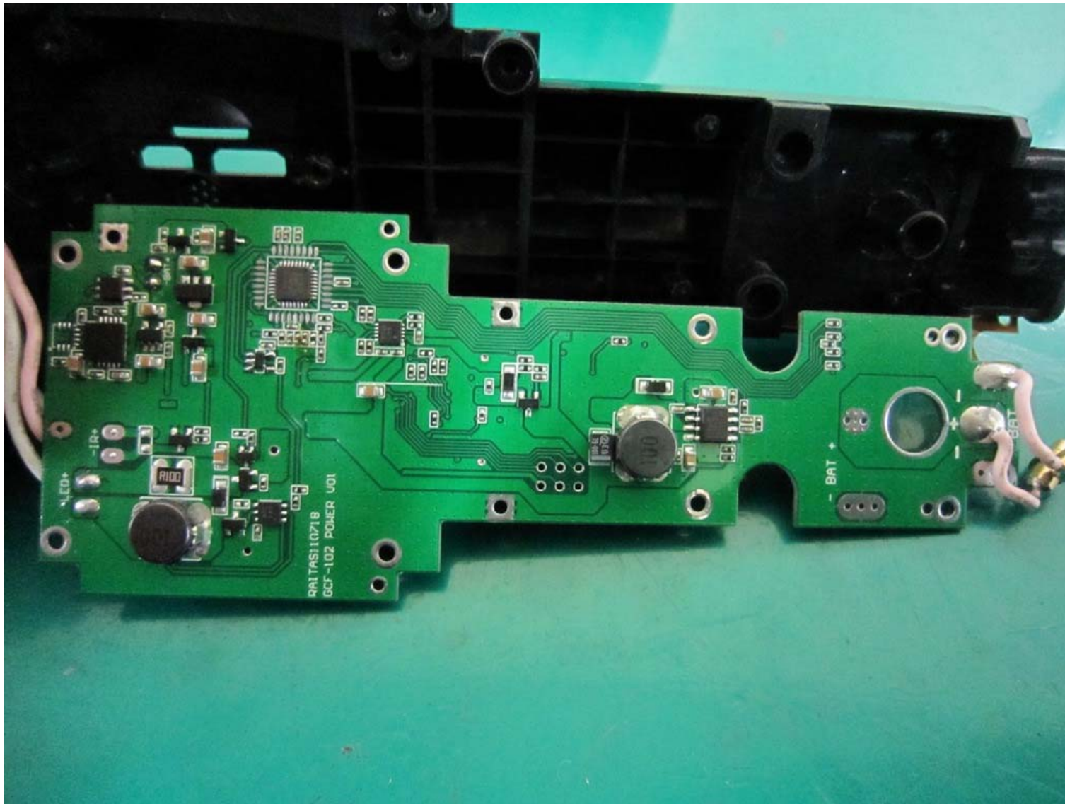
GCF-200_Power Board(Front View)
