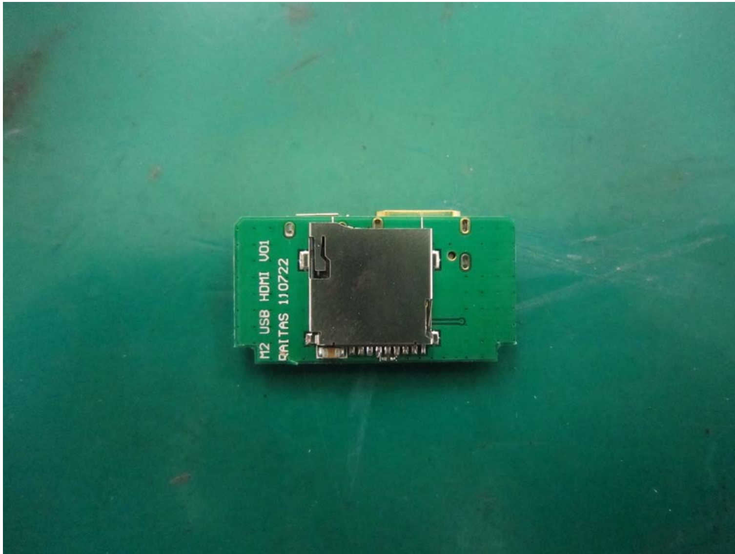
GCF-200_Interface Board(Rear View)
