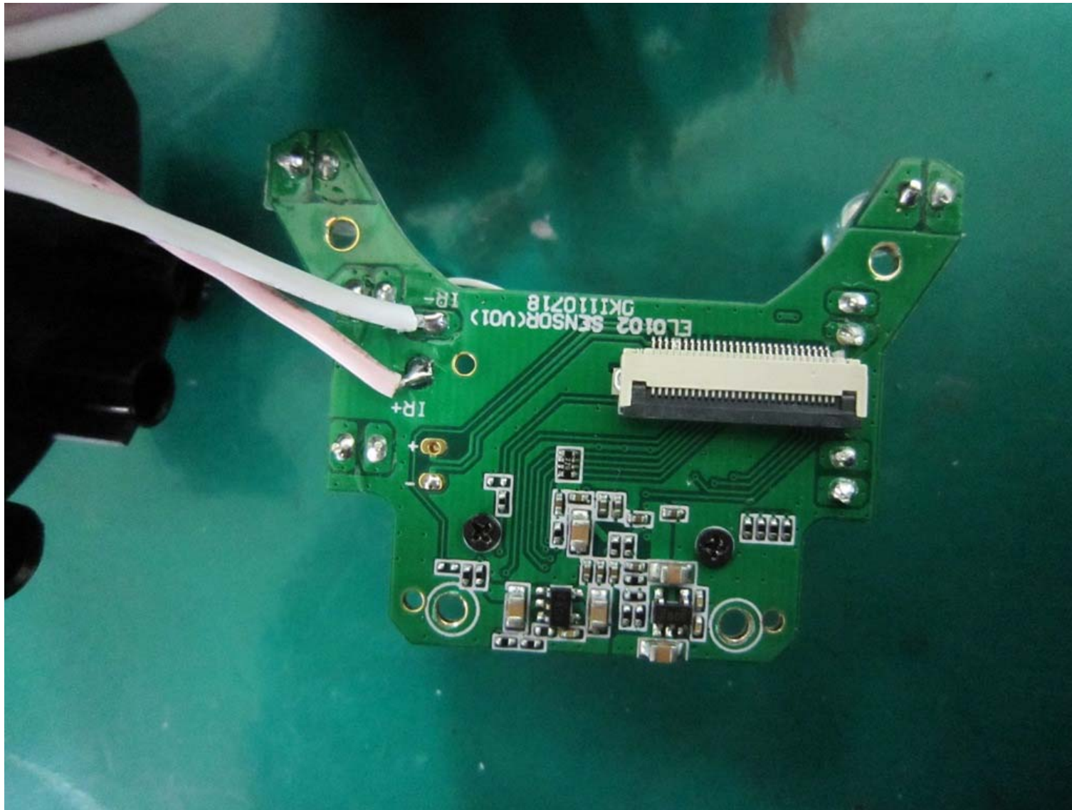
GCF-200_Camera Board(Rear View)
