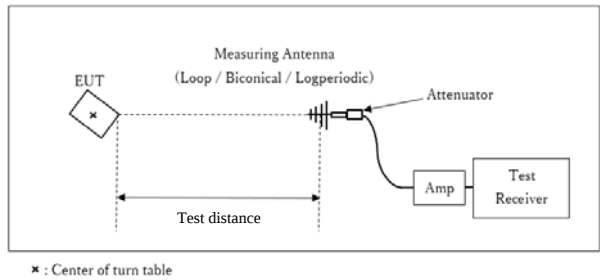
Figure 3: Test Setup
