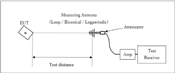
Figure 3: Test Setup
