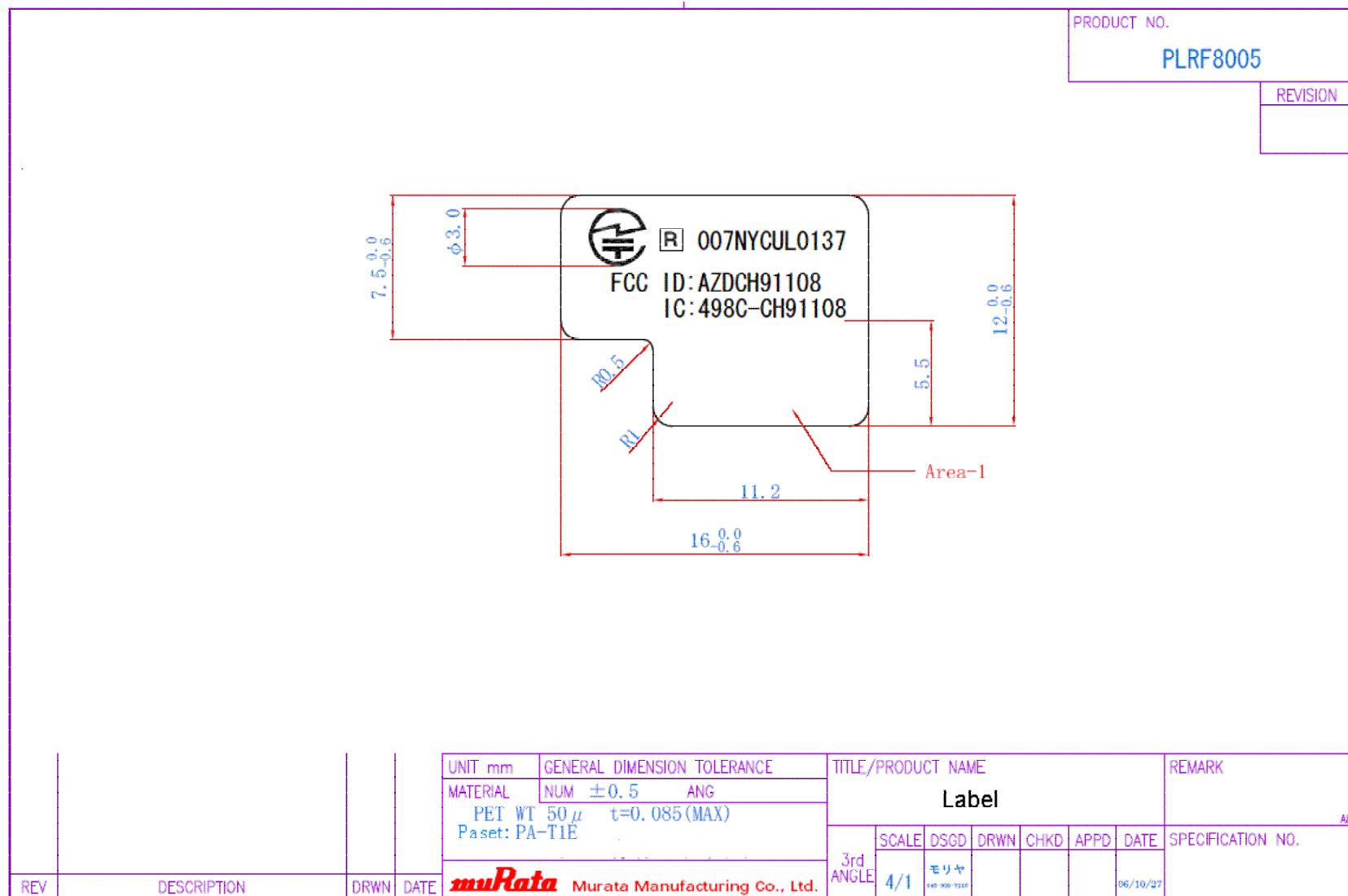
Fig1. Dimension of Label
