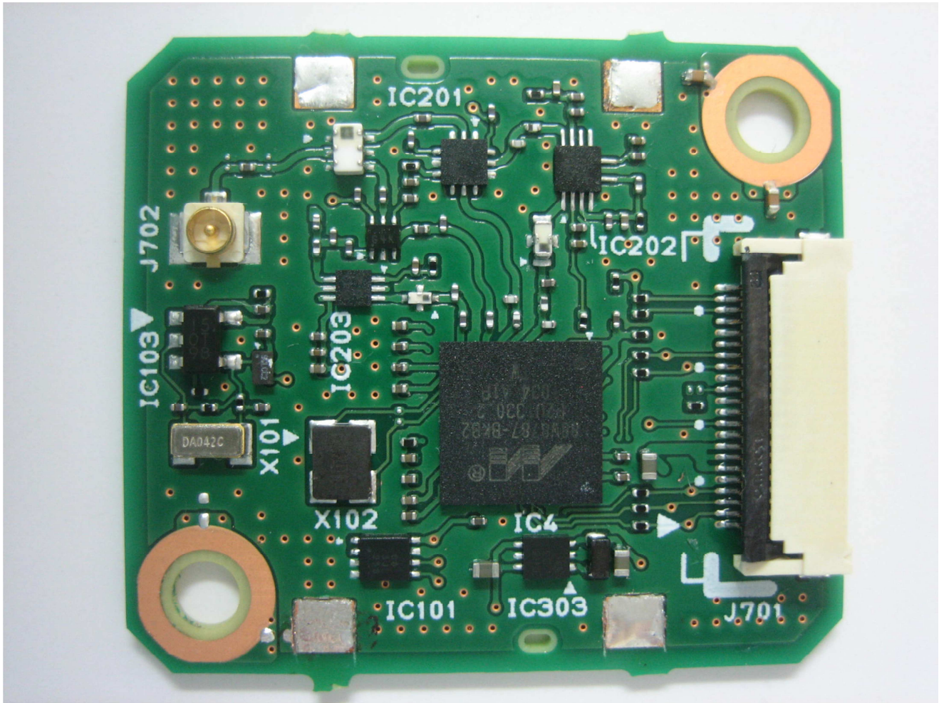
Component Side (without Shield)
