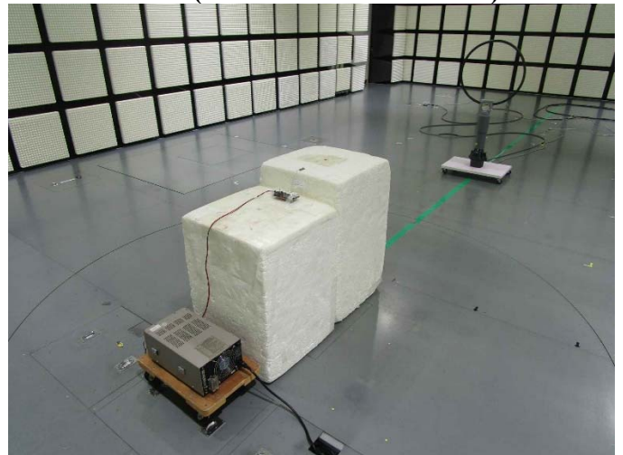
Rear (Below 30 MHz Vertical)
