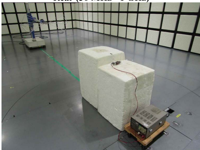
Rear (30 MHz - 1 GHz)
