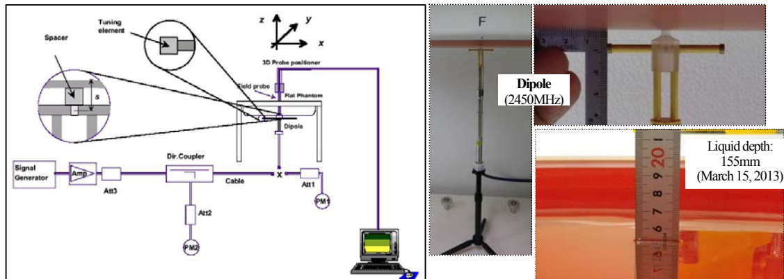
Test setup for the system performance check
