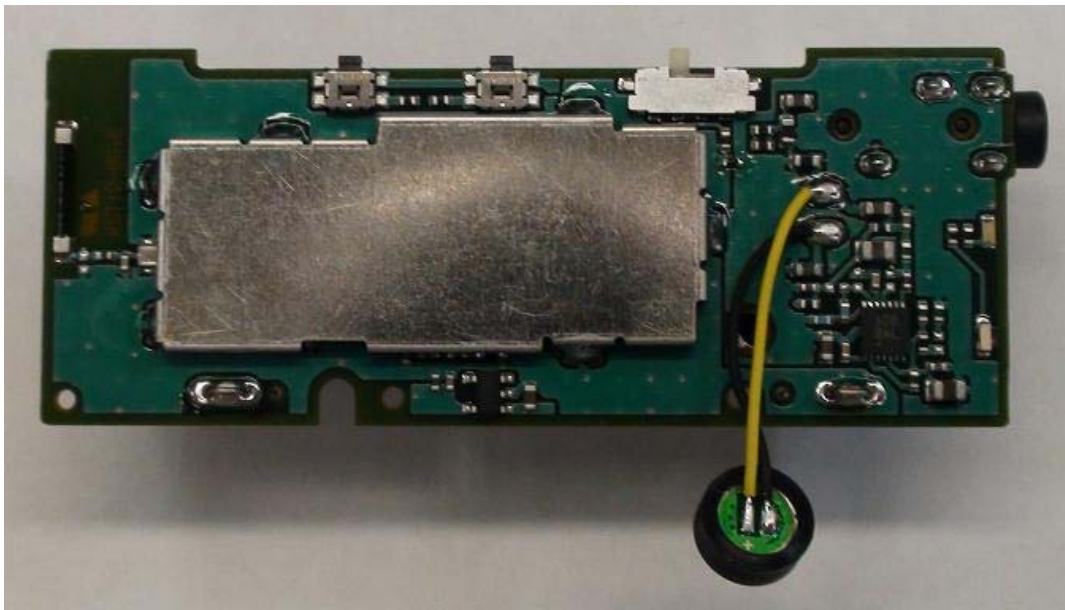
Top (with shield case)
