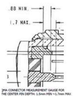
Figure 1C – Tolerance of QMA center pin
