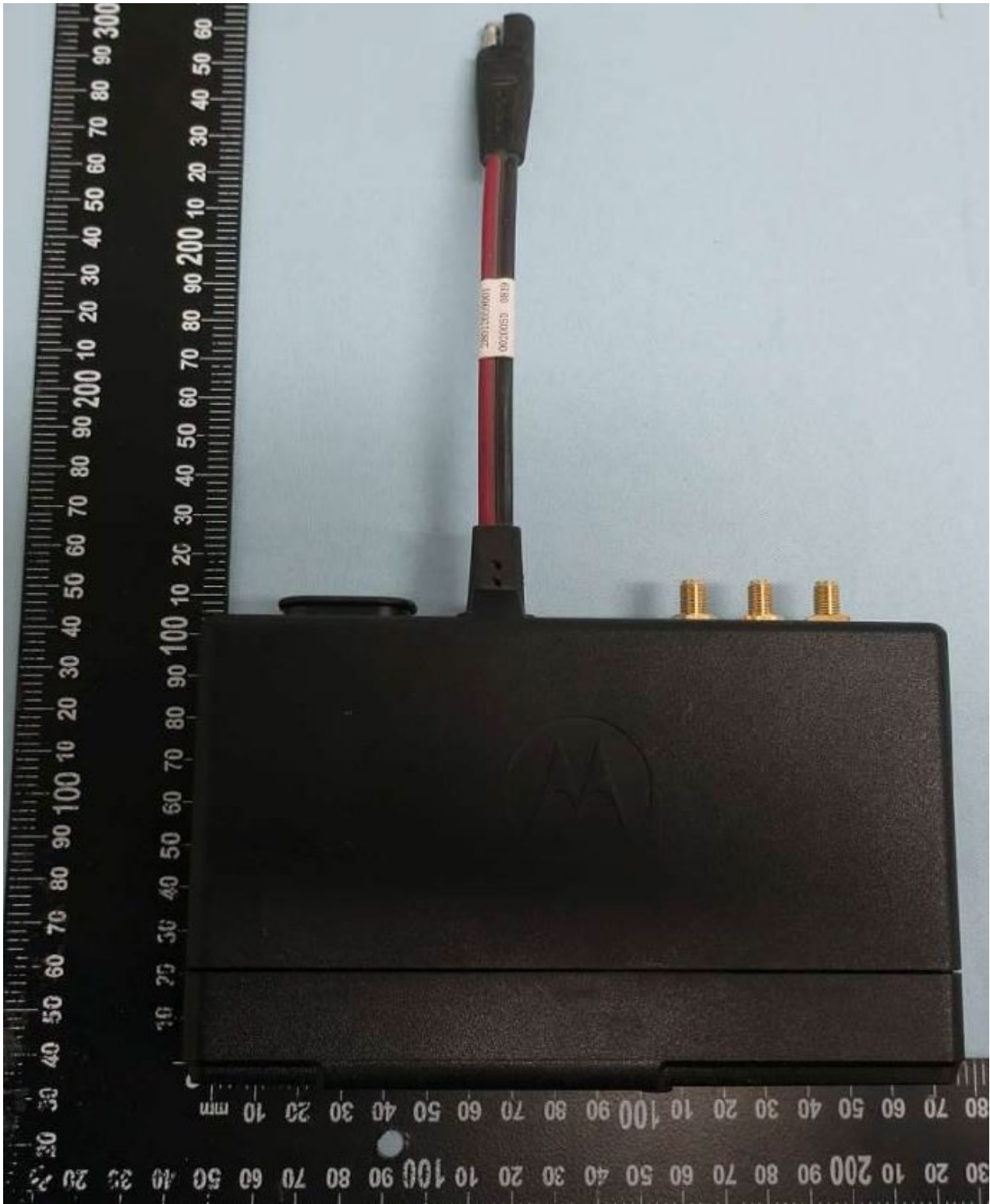
Top View
