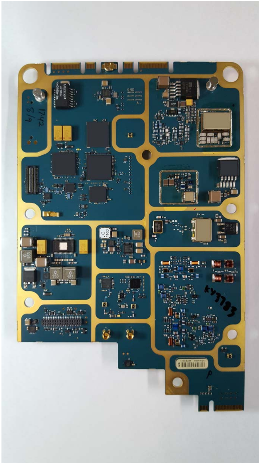
Exhibit 9E: Transceiver Board without Shields (Top)
