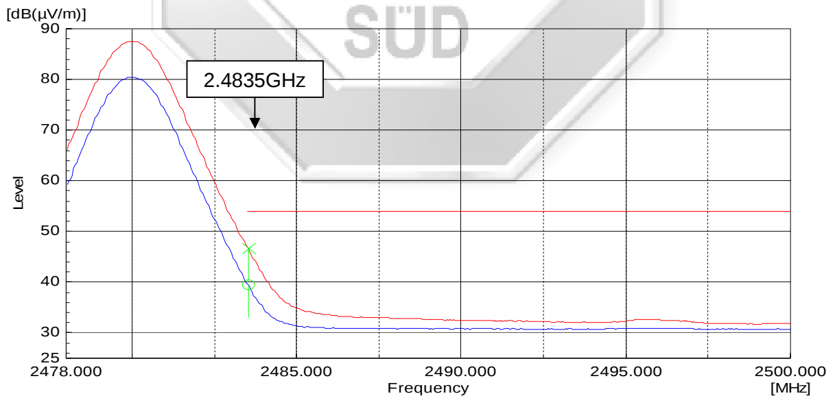
Plot 71 – Average Plot at Upper Band Edge at 2.4835GHz
