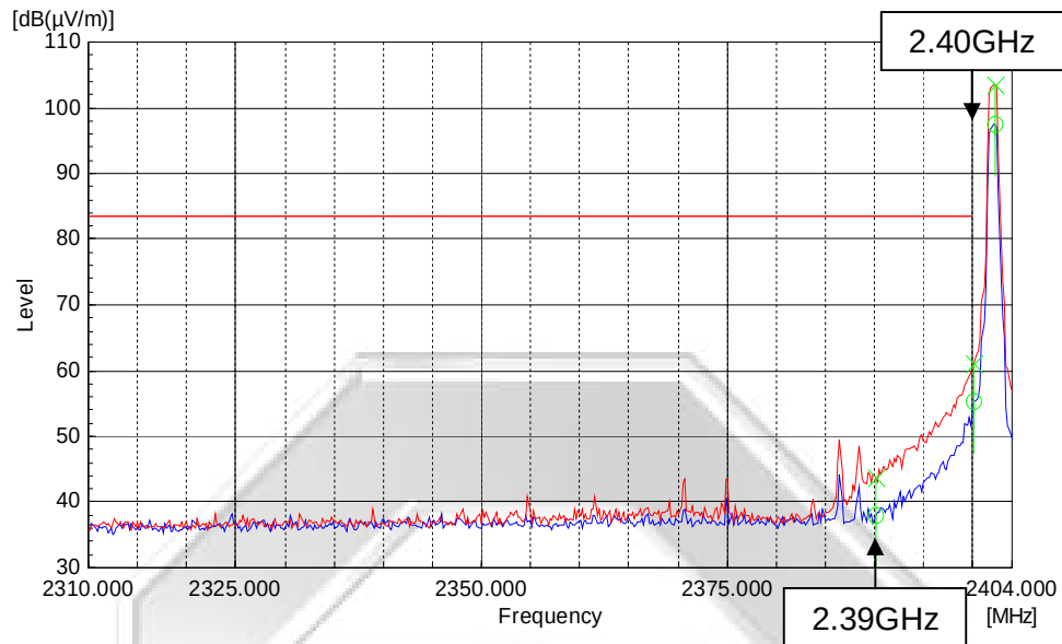
Plot 33 – Lower Band Edge at 2.4000GHz
