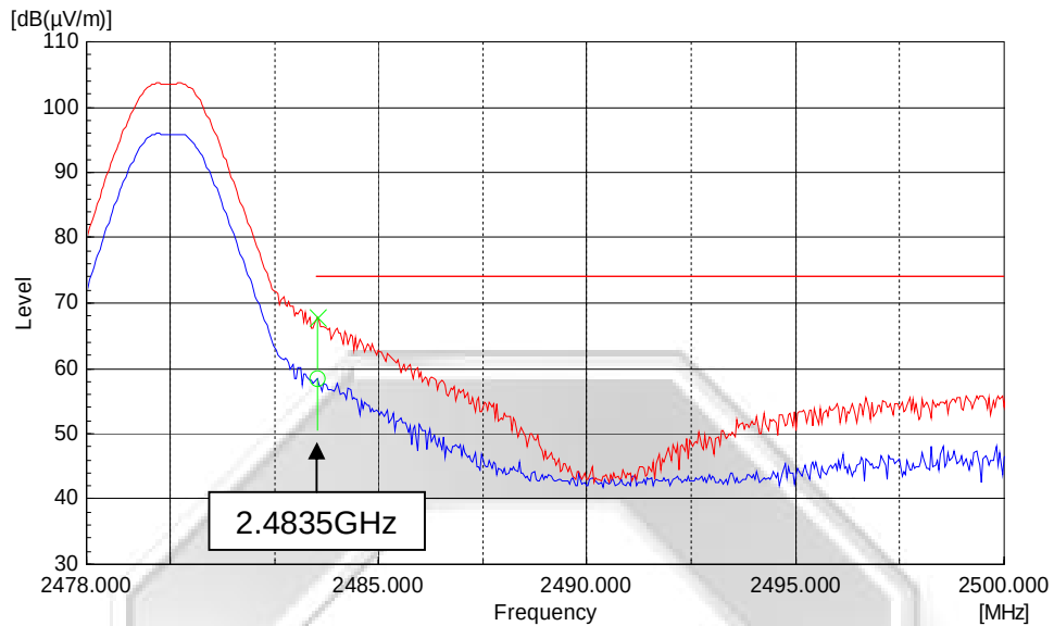
Plot 37 – Peak Plot at Upper Band Edge at 2.4835GHz
