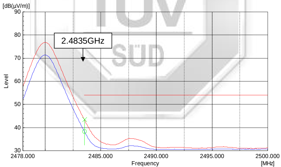
Plot 38 – Average Plot at Upper Band Edge at 2.4835GHz
