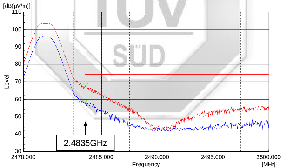
Plot 34 – Upper Band Edge at 2.4835GHz
