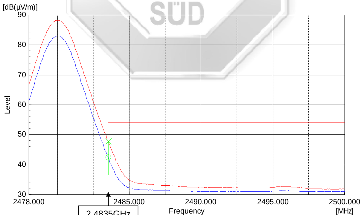
Plot 71 – Average Plot at Upper Band Edge at 2.4835GHz
