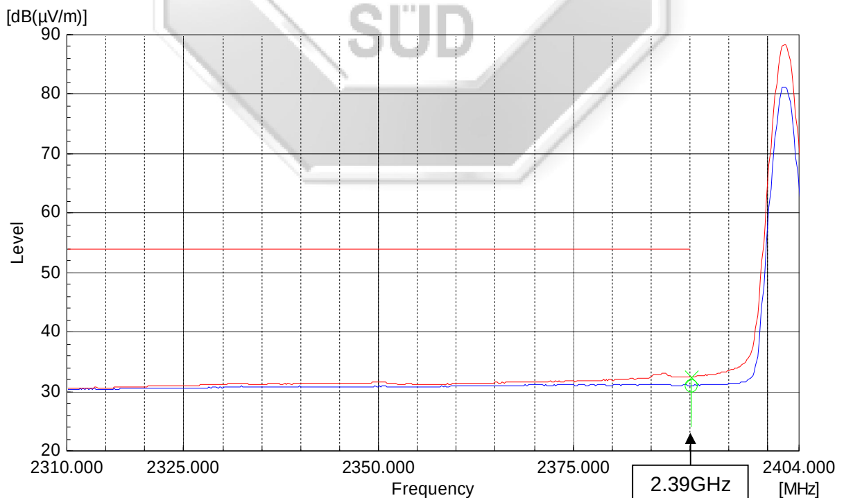
Plot 69 – Average Plot at Lower Band Edge at 2.4000GHz
