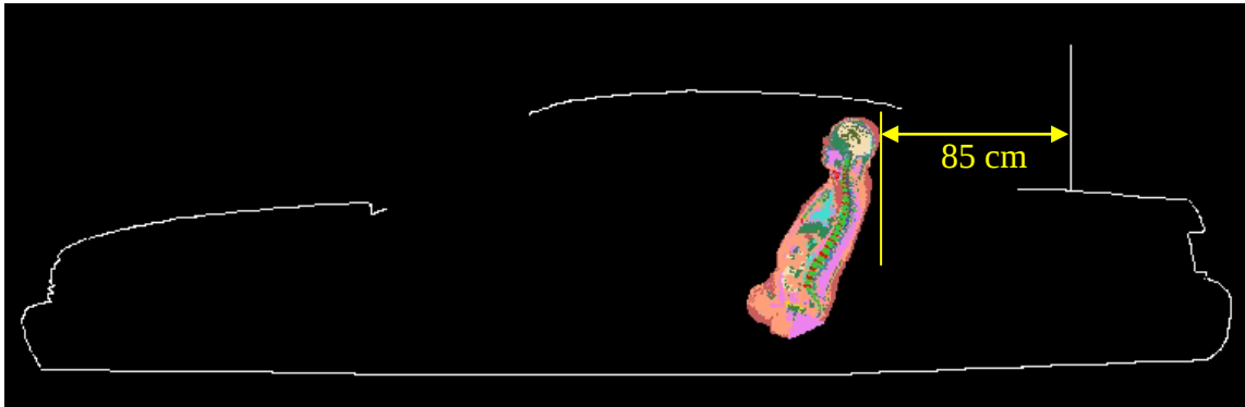
Figure 3: Passenger model exposed to a trunk-mount antenna: XFDTD geometry. The antenna is mounted at 85 cm from the passenger located in the center of the back seat.
