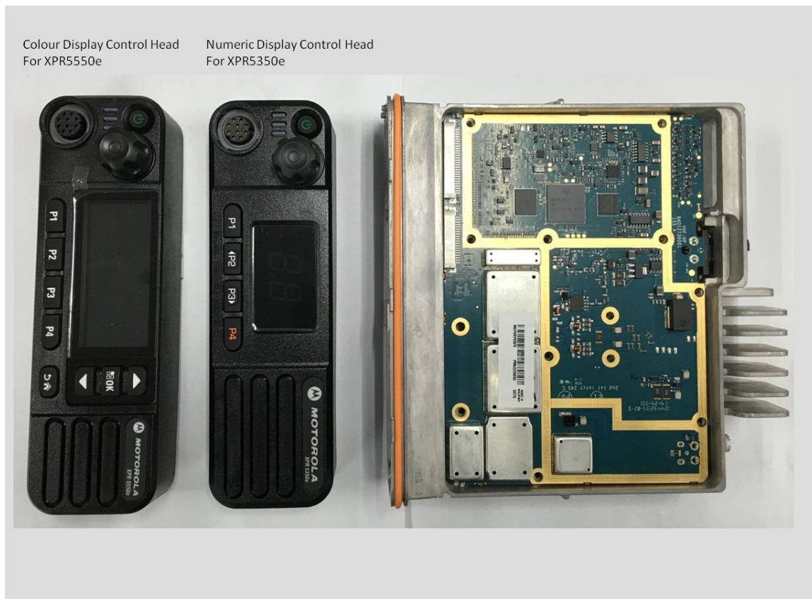
Chassis and control heads (Top)
