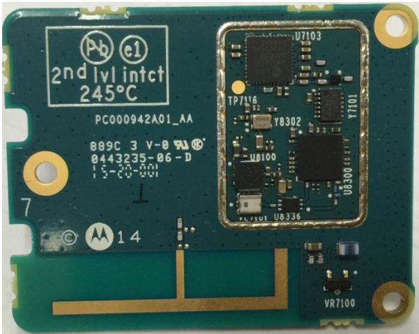
GPS/BT/Wifi board without shield (Bottom)
