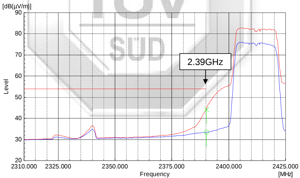
Plot 368 – Average Plot at Lower Band Edge at 2.4000GHz @ 64QAM 65Mbps
