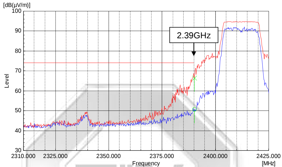
Plot 361 – Peak Plot at Lower Band Edge at 2.4000GHz @ 64QAM 54Mbps
