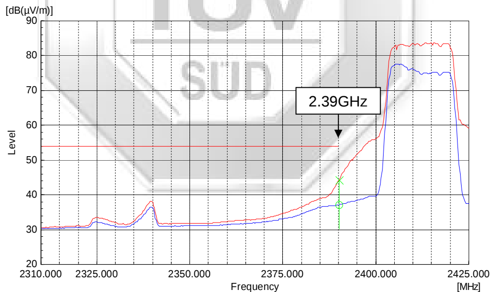
Plot 362 – Average Plot at Lower Band Edge at 2.4000GHz @ 64QAM 54Mbps
