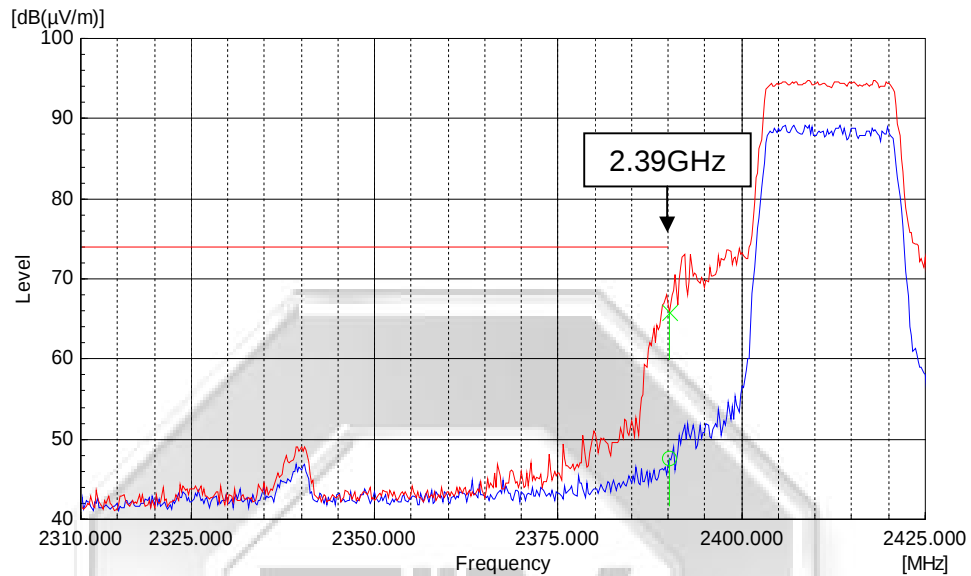
Plot 367 – Peak Plot at Lower Band Edge at 2.4000GHz @ 64QAM 65Mbps
