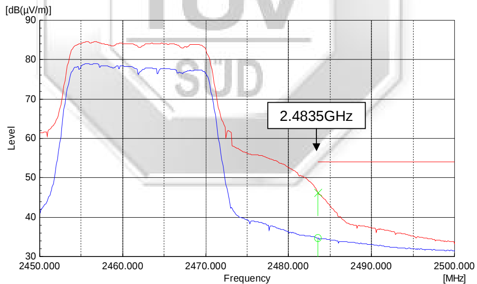
Plot 364 – Average Plot at Upper Band Edge at 2.4835GHz @ 64QAM 54Mbps
