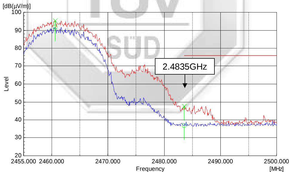
Plot 354 – Upper Band Edge at 2.4835GHz @ CCK 11Mbps
