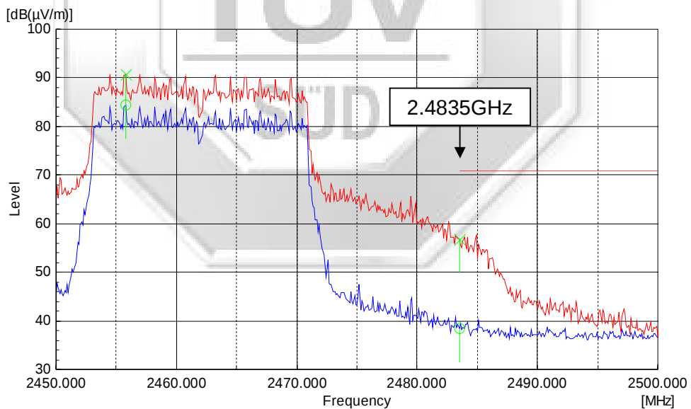
Plot 366 – Upper Band Edge at 2.4835GHz @ 64QAM 65Mbps
