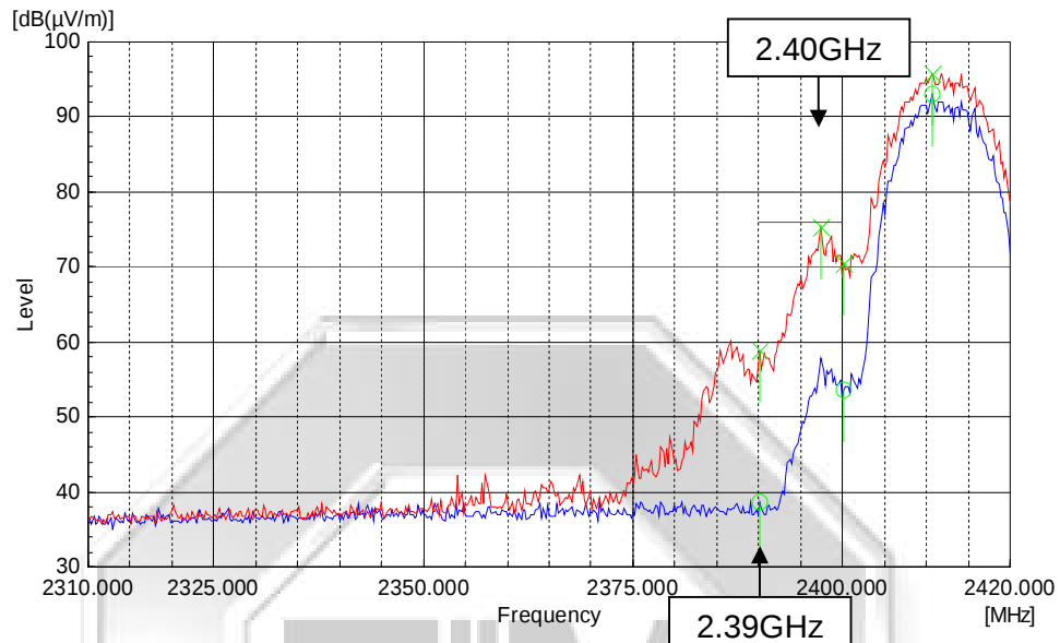
Plot 353 – Lower Band Edge at 2.4000GHz @ CCK 11Mbps
