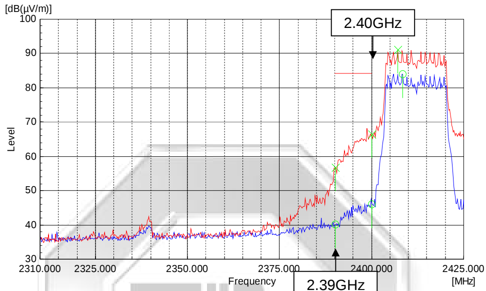
Plot 359 – Lower Band Edge at 2.4000GHz @ 64QAM 54Mbps
