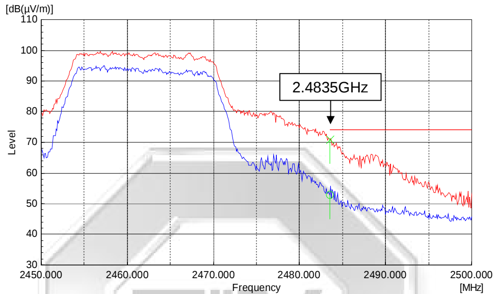
Plot 363 – Peak Plot at Upper Band Edge at 2.4835GHz @ 64QAM 54Mbps
