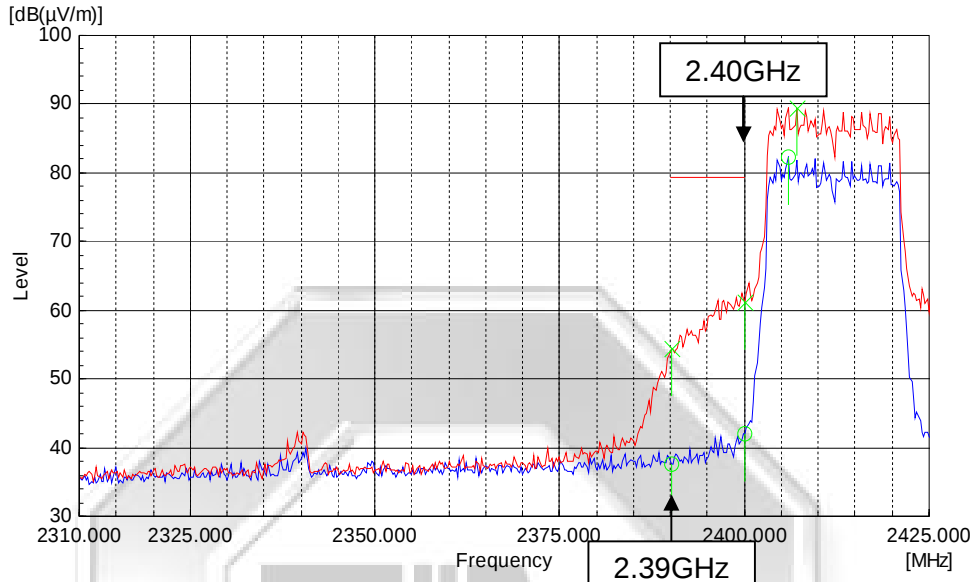
Plot 365 – Lower Band Edge at 2.4000GHz @ 64QAM 65Mbps
