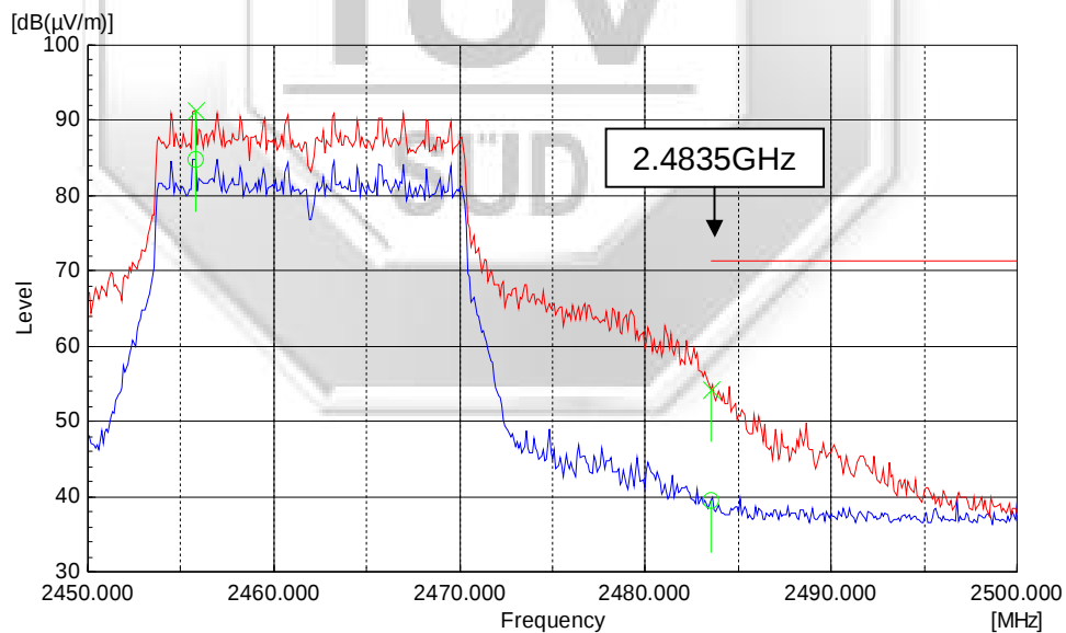
Plot 360 – Upper Band Edge at 2.4835GHz @ 64QAM 54Mbps
