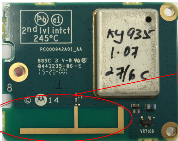
GPS/BT/Wifi board with shield (Bottom)
