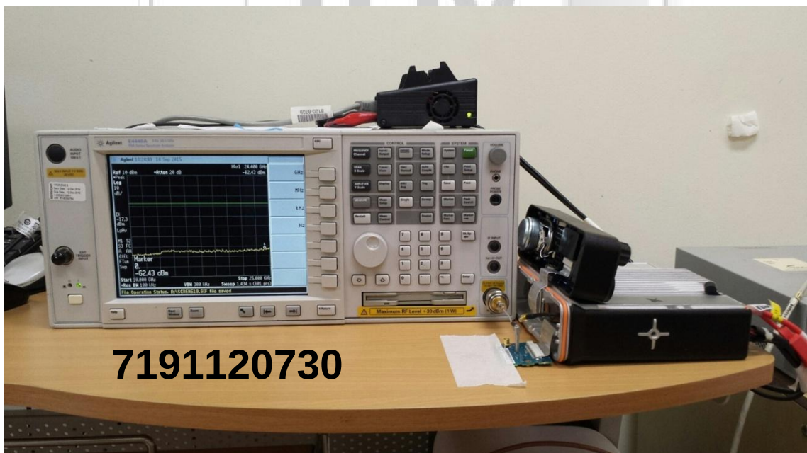
Average Frequency Dwell Time Test Setup
