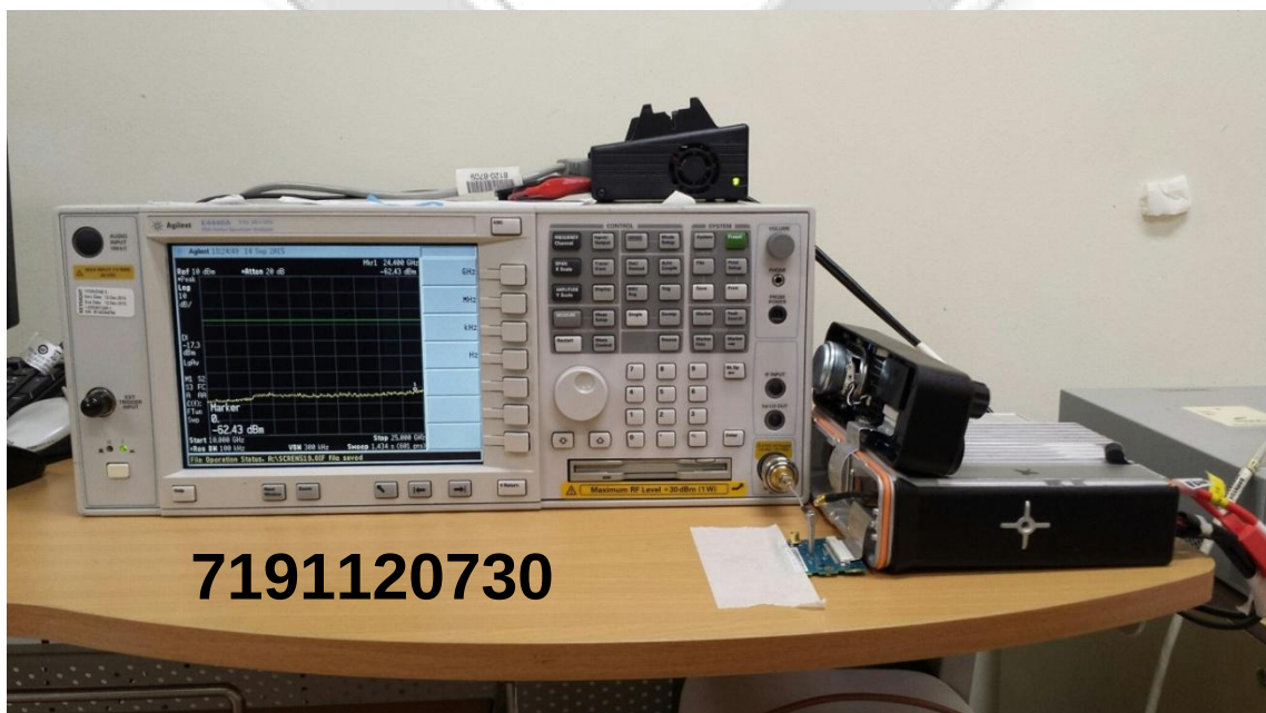
RF Conducted Spurious Emissions Test Setup
