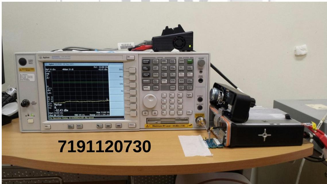
Spectrum Bandwidth (20dB Bandwidth Measurement) Test Setup
