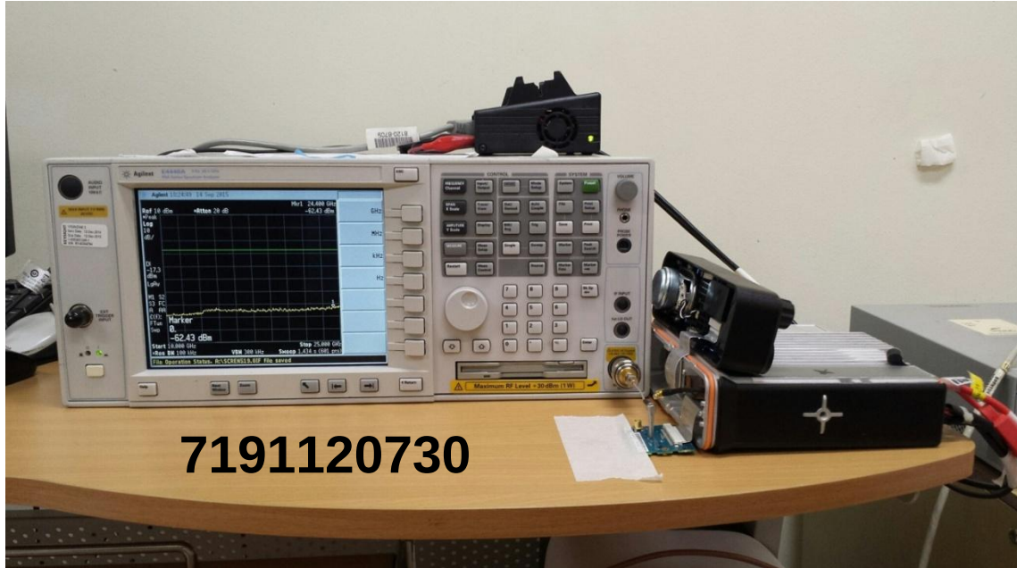
Carrier Frequency Separation Test Setup
