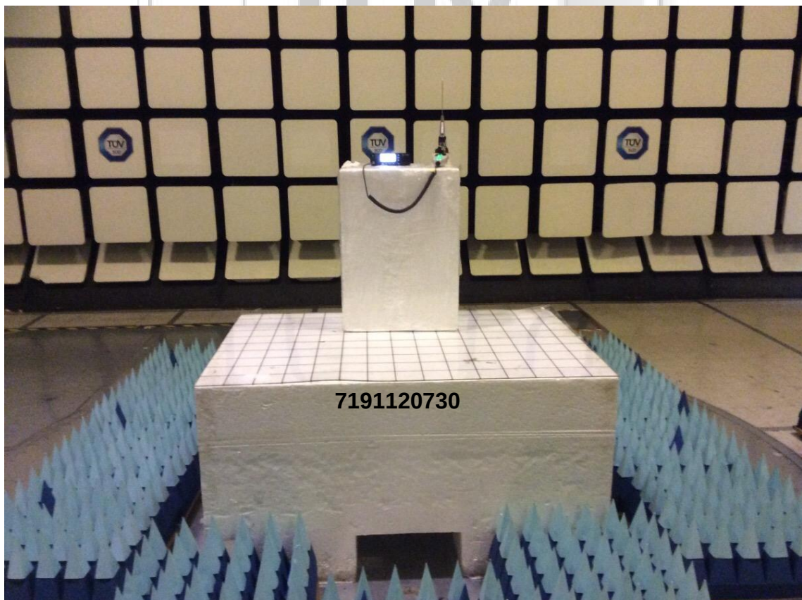
Band Edge Compliance (Radiated) Test Setup
