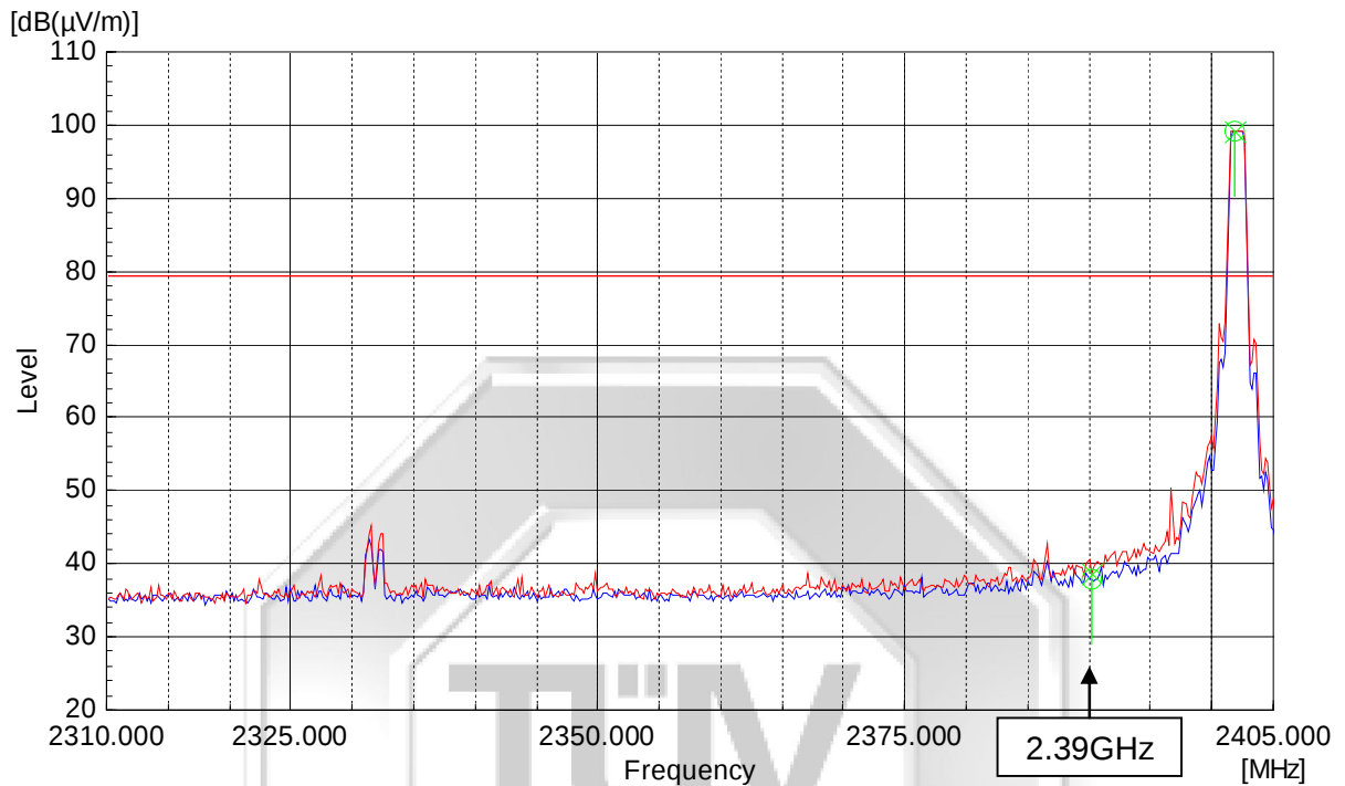
Plot 66 – Lower Band Edge at 2.4000GHz
