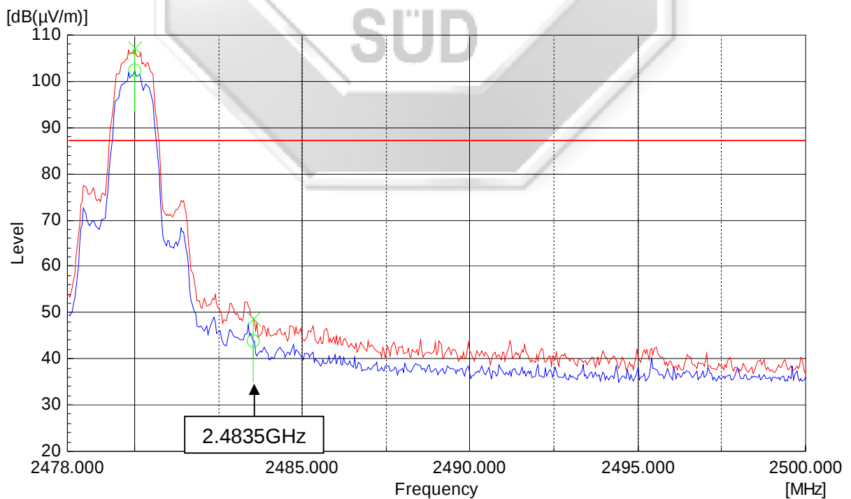
Plot 67 – Upper Band Edge at 2.4835GHz
