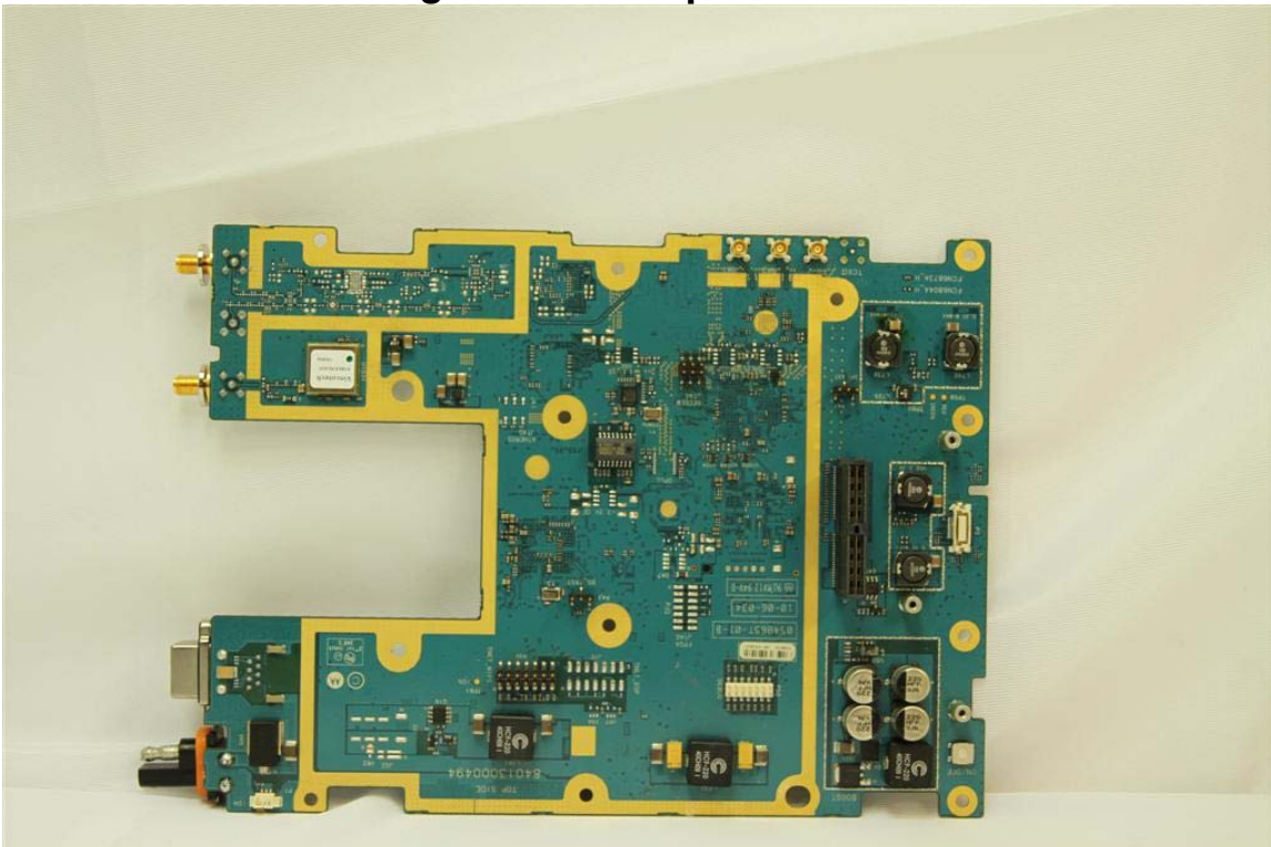
Figure No.2 VM2500 – Digital Board top view without shield
