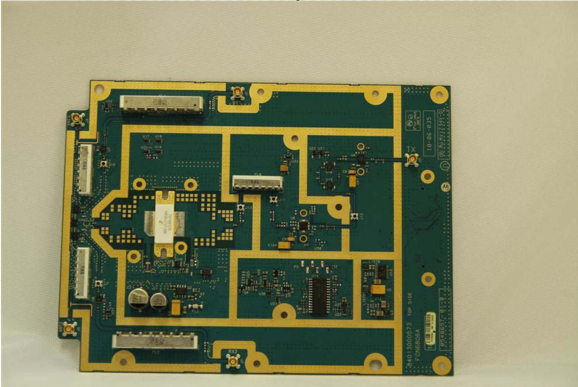
Figure No.6 VM2500 – RF Board top view without shield
