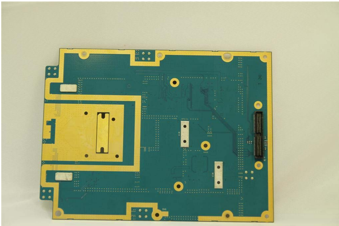
Figure No.5 VM2500 – RF Board bottom view without shield
