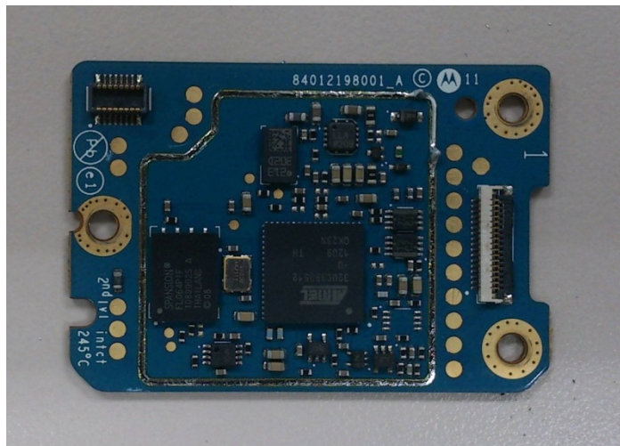
GOB board without shield (Bottom)
