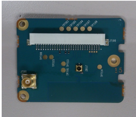
GPS/BT board (Top)
