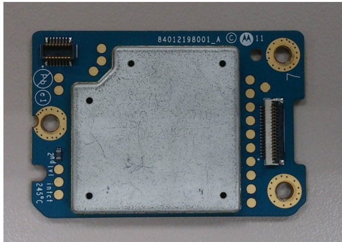
GOB board with shield (Bottom)
