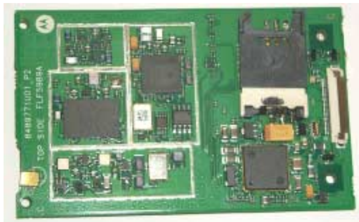
Photograph 9-2: Front side of module main board with shields removed.
