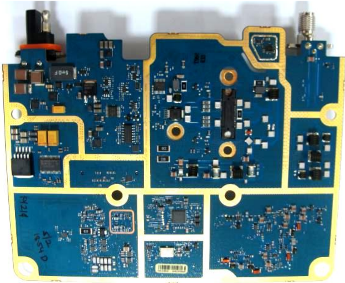
RF board without Shields (Bottom)
