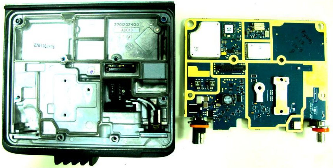
RF board with chassis assembly
