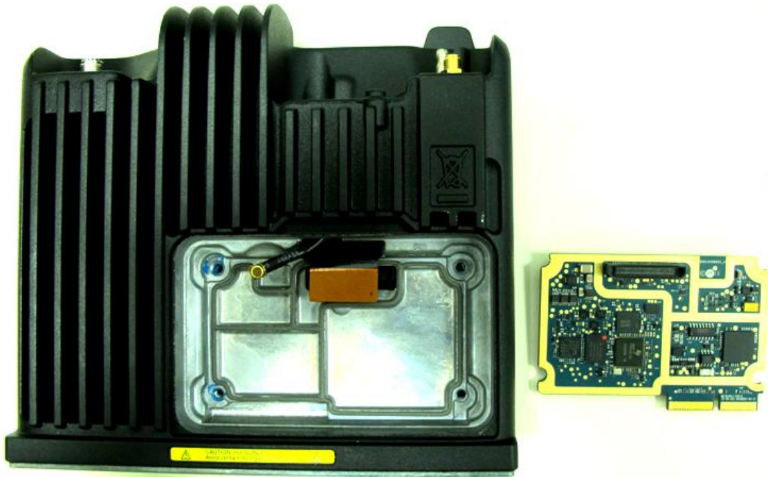
Controller board with chassis assembly
