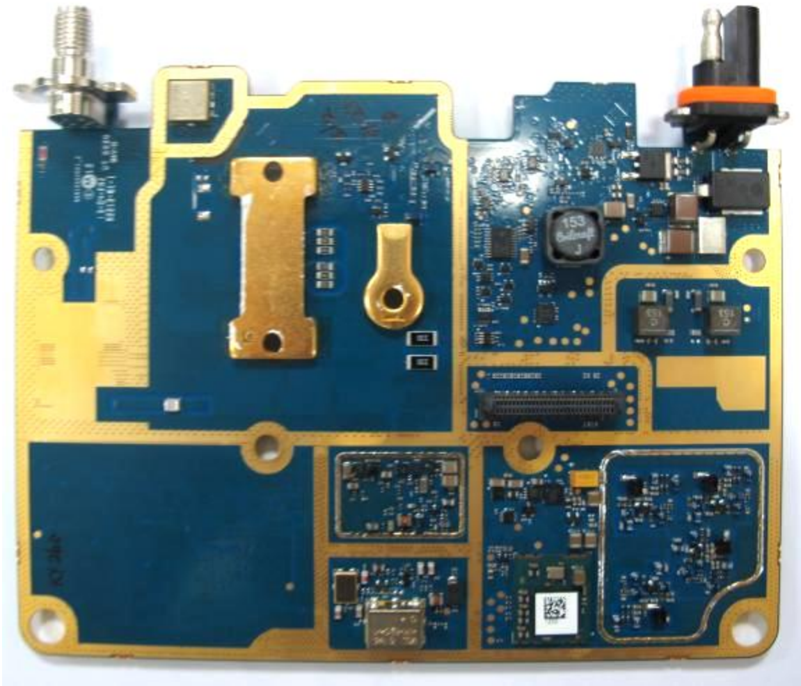
RF board without Shields (Top)
