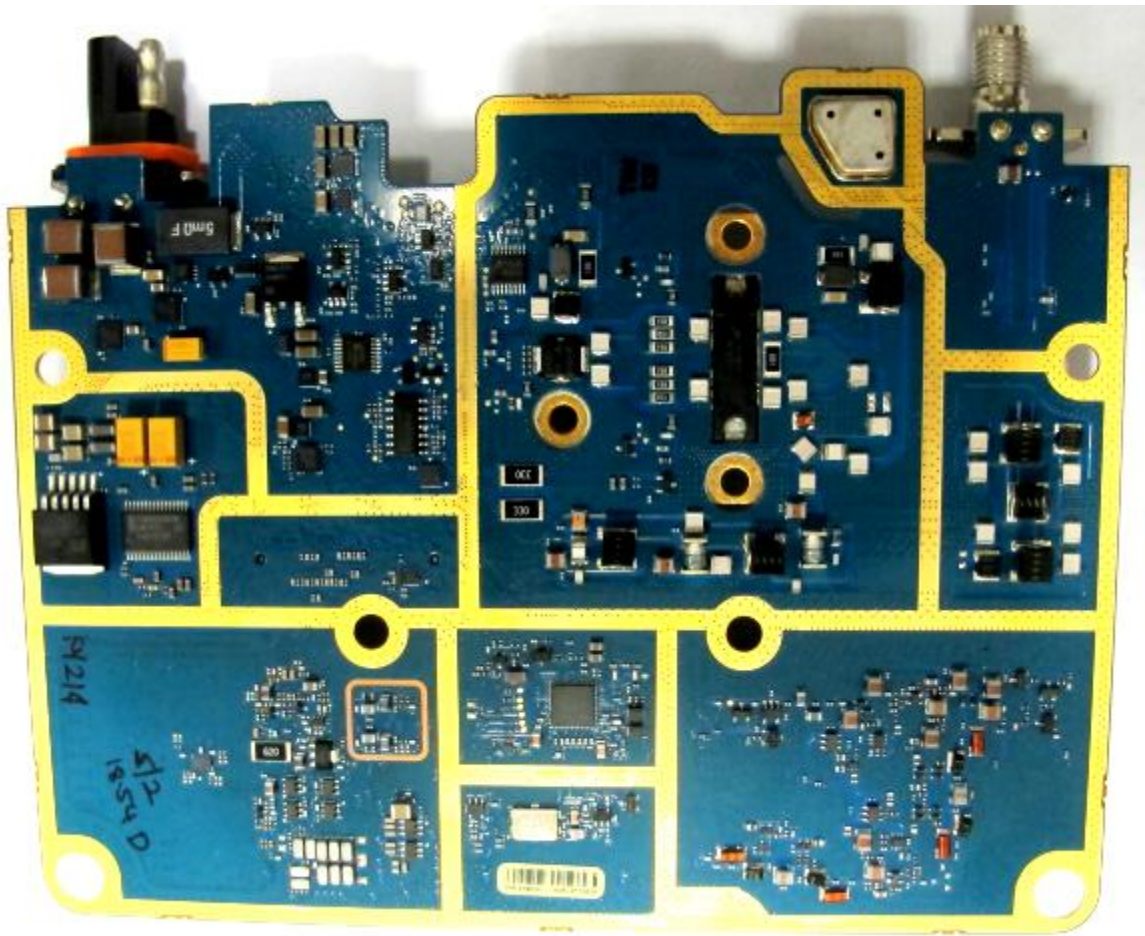
RF board with Shields (Bottom)
