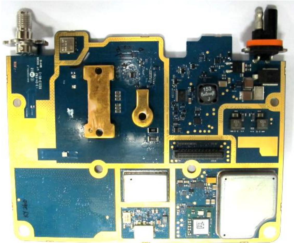
RF board with Shields (Top)
