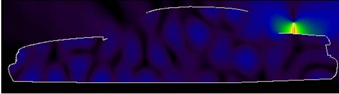
Figure 5 (a) E-field distribution and (b) H-field distribution in the plane of the trunk mounted antenna (HAE4003A antenna at 450 MHz) corresponding to the passenger exposure condition
