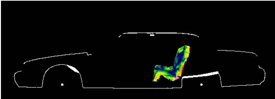
Figure 3: SAR distribution at 450 MHz in the passenger located on the side of the back seat, produced by the trunk-mount HAE6031A antenna. The contour plot in the figure is relative to the plane where the peak 1-g average SAR for this exposure condition occurs.
