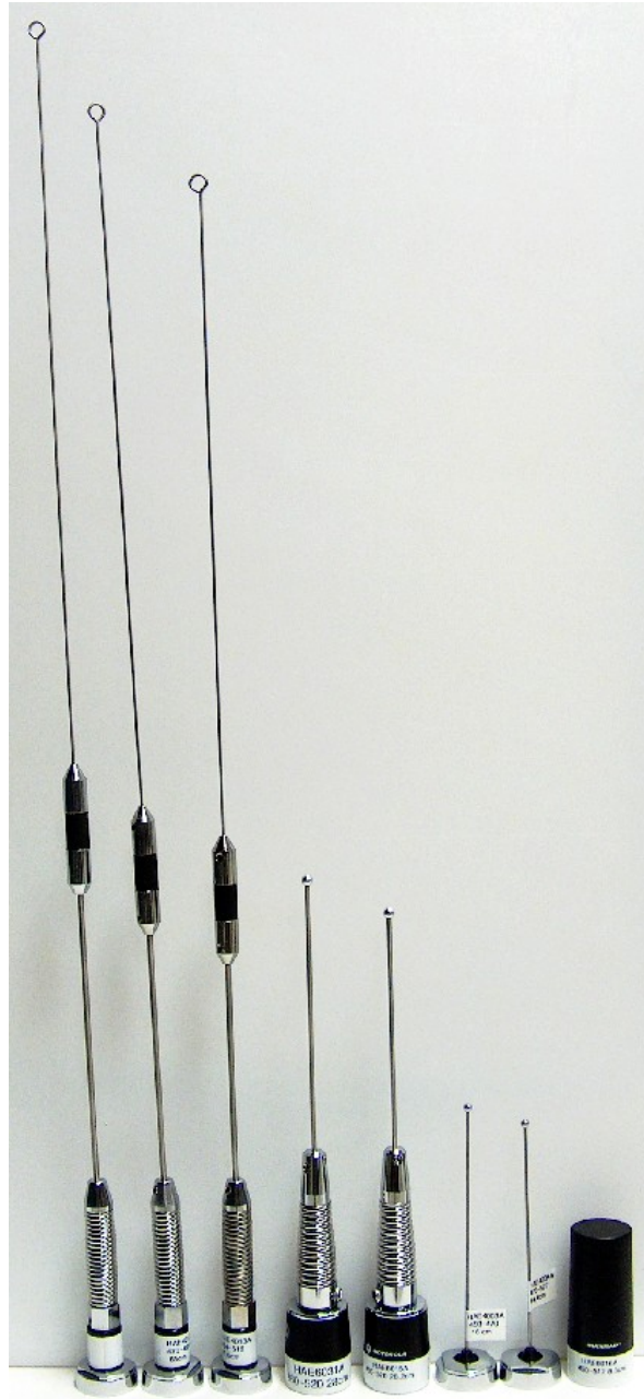
UHF R2 Antenna kit numbers, from left to right: HAE4011A, HAE4012A, HAE4013A, HAE6031A, HAE6015A, HAE4003A, HAE4004A & HAE6016A
