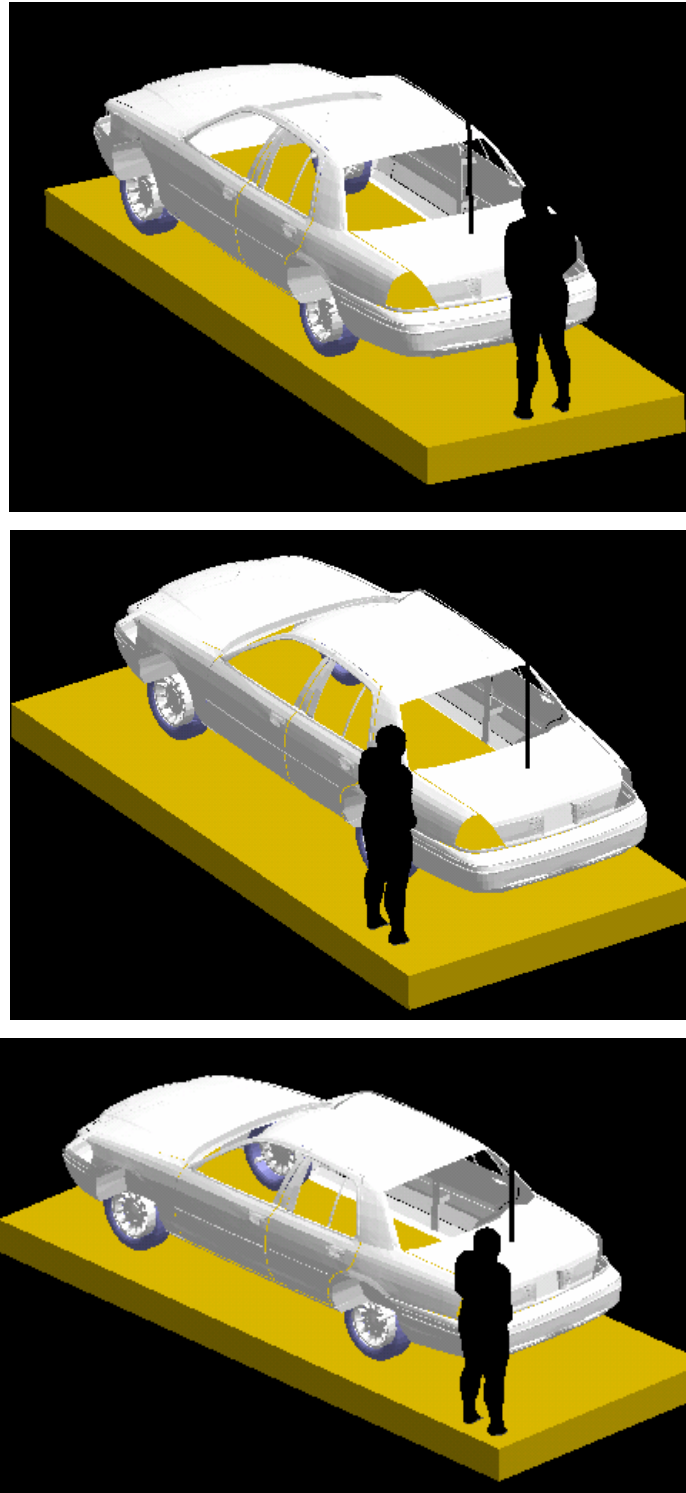
Figure 1: Bystander model exposed to a trunk-mount VHF antenna: Bystander is located at the back, on the side or at the corner of the car replicating the measurement conditions. The antenna is mounted in the center of the trunk. The dielectric slab under the car is introduced to model the ground (pavement) effect on exposure.
