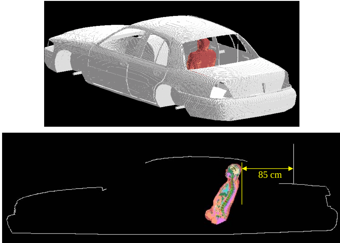
Figure 2: Passenger model exposed to a trunk-mount antenna: XFDTD geometry. The antenna is mounted at 85 cm from the passenger located in the center of the back seat.
