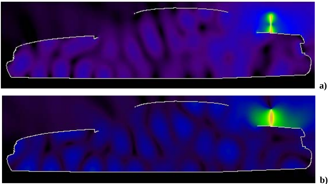
Figure 4 (a) E-field distribution corresponding to exposure condition of Figure 3, and (b) H-field distribution corresponding to exposure condition of Figure 3.
