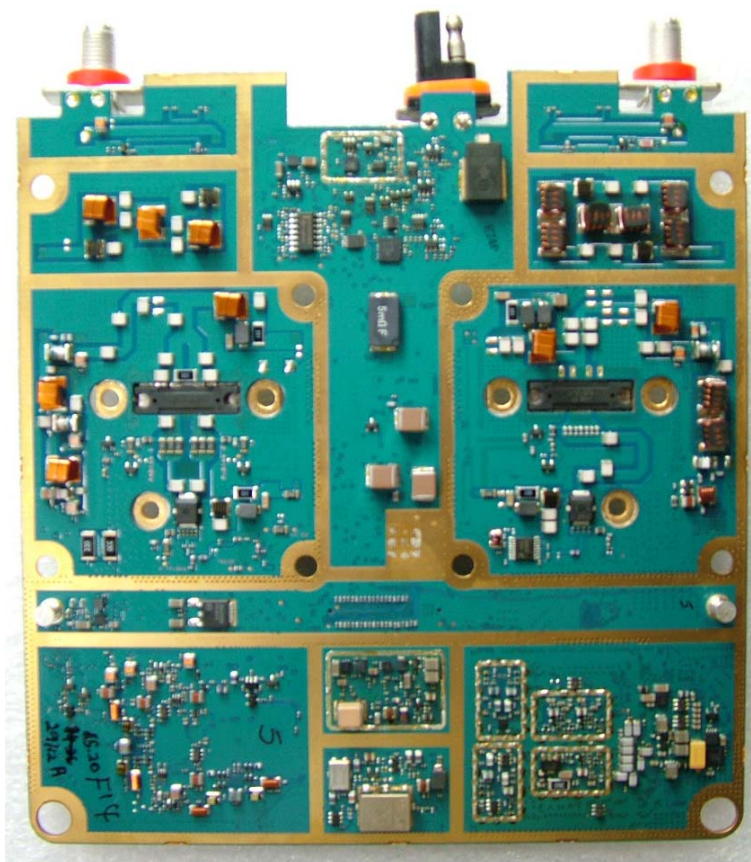
RF board without Shields (Top)
