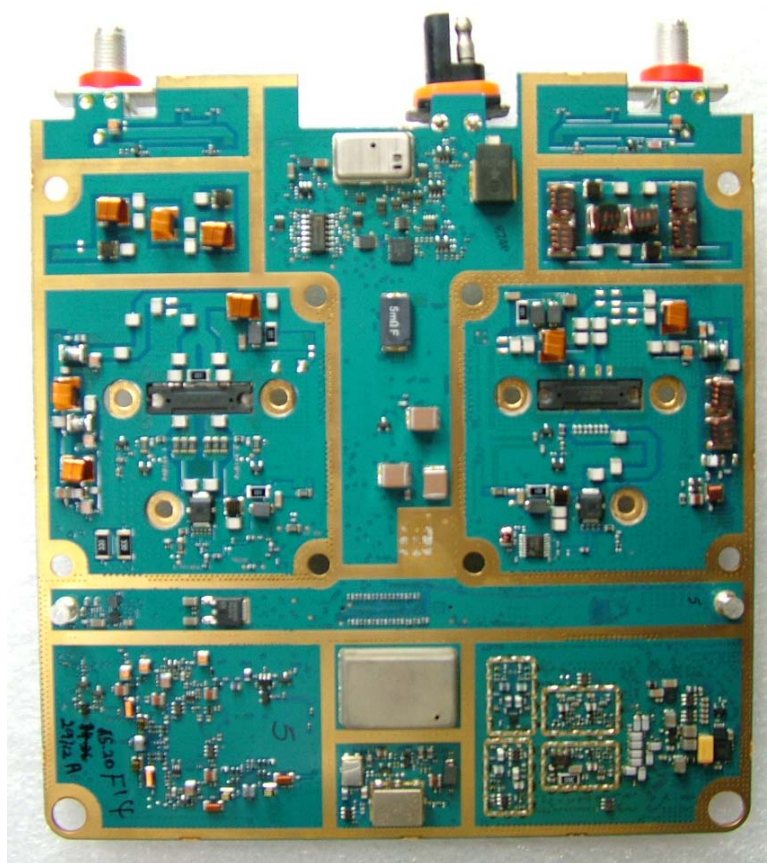
RF board with Shields (Top)
