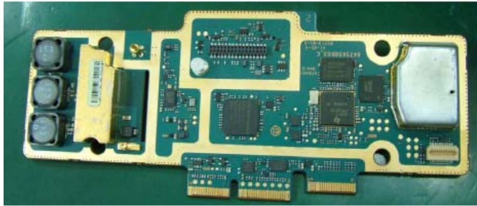
Controller board with Shields (Bottom)
