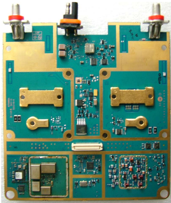
RF board with Shields (Bottom)
