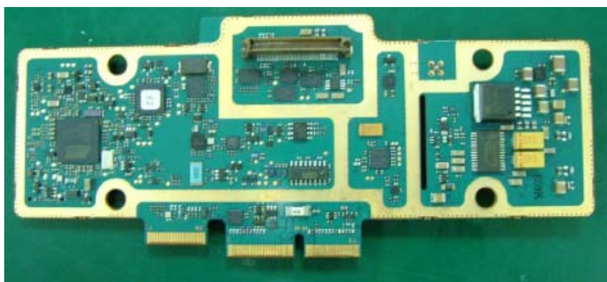
Controller board with Shields (Top)
