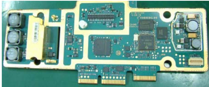
Controller board without Shields (Bottom)
