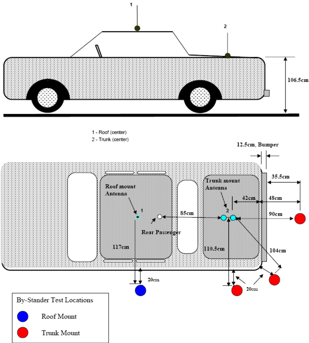
Antenna Location Drawing with Test Locations Identified
