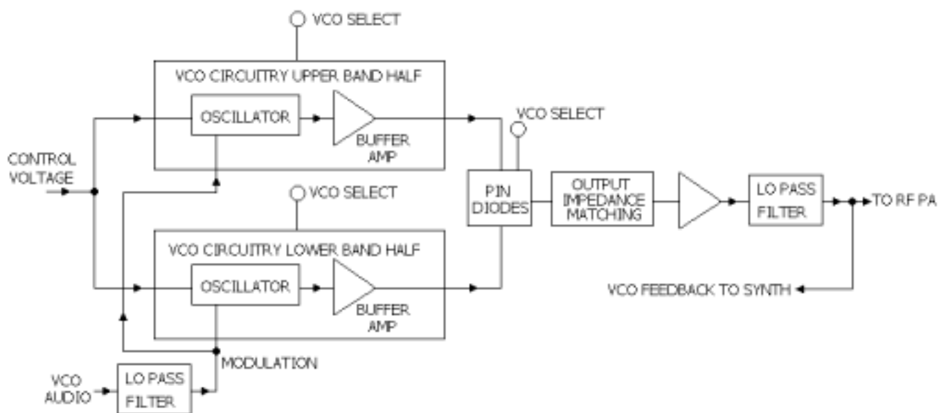
Figure 3: VCO Circuitry
