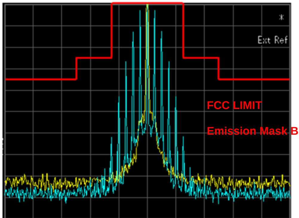
Figure 6E-8: 159.7625 MHz, 25 kHz Channel Spacing (Analog Voice), Mask B 16K0F3E (Part 80.205)
