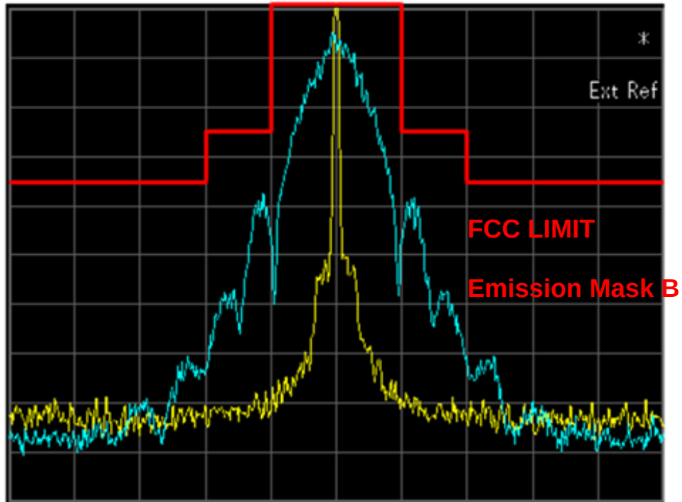
Figure 6E-9: 159.7625 MHz, 20 kHz Channel Spacing (Analog Voice Encryption) (Part 80.205)
