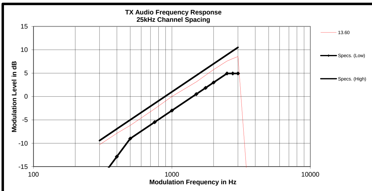
Figure 6B-2: 25 kHz Channel Spacing, 154.9875 MHz (Not for FCC Review)
