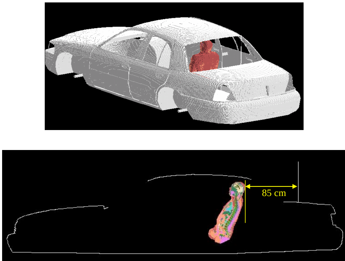
Figure 2: Passenger model exposed to a trunk-mount antenna: XFDTD geometry. The antenna is mounted at 85 cm from the passenger located in the center of the back seat.
