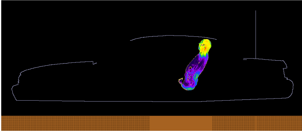
Figure 3. SAR distribution at 173.4 MHz in the passenger model located in the center of the back seat, produced by the trunk-mount HAD4022A antenna. The contour plot is relative to the plane where the peak 1-g average SAR for this exposure condition occurs.
