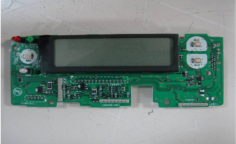
Figure 9.9: LCD display front view
