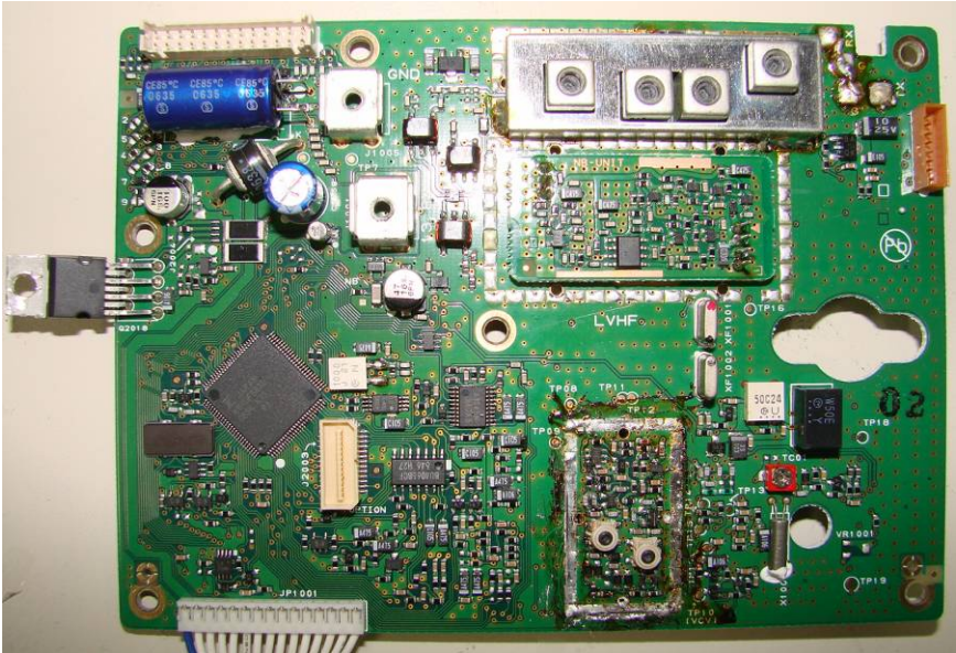
Figure 9.3: RF controller unit front view (without shield)
