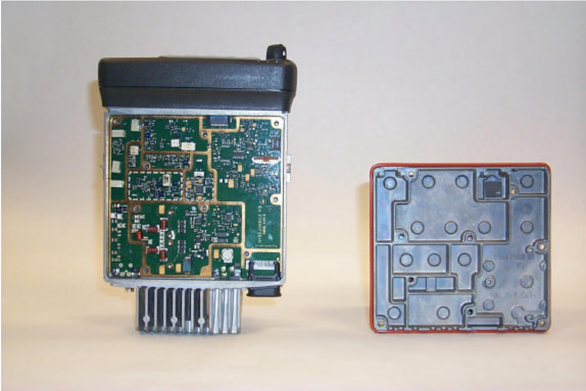
TOP VIEW, WITH METAL SHIELD COVER REMOVED (TOP SIDE OF CIRCUIT BOARD VISIBLE)
